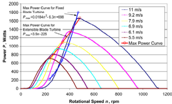
Fig. 5 Power curves for turbine with variable length blades [14].
