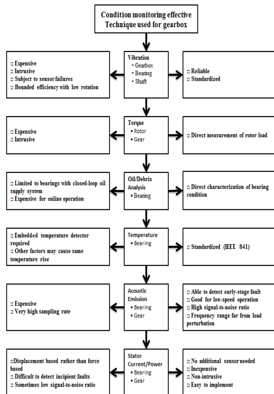
Fig. 2 Gearbox Condition monitoring Techniques.
