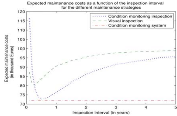
Fig.(6) Expected maintenance costs for the different maintenance strategies as a function of the inspection interval t_1 for the case study (one blade) [15].
