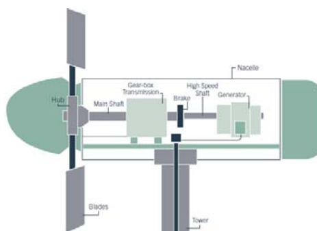
Figure (3): Diagram showing the inside of the nacelle(main components)[17].
