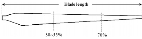
Figure (4) : The spanwise location of a blade that is likely to damage [11].
