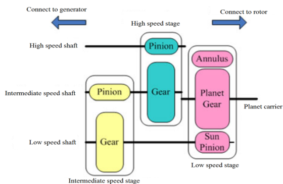
Fig.1. Gearbox Structure [8]
