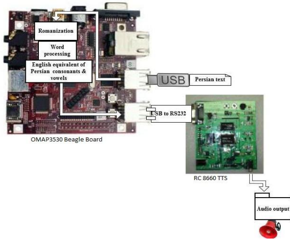
Figure 2. Beagle board (omap3530) as an application processor RC8660 as an integrated TTS processor
