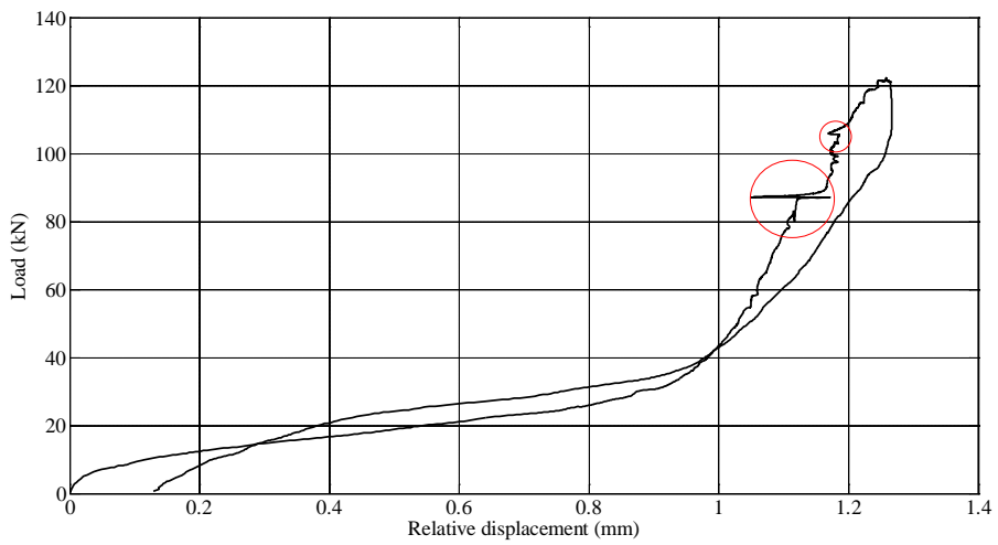
Figure 15 - Load-deformation curves in the first loading scenario (a) Load-vertical deflection curve for D2, (b) Load-relative displacement curve for S2
