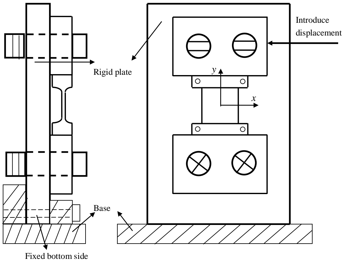
Figure 4 - A platform used to calibrate the sensor sensitivity
