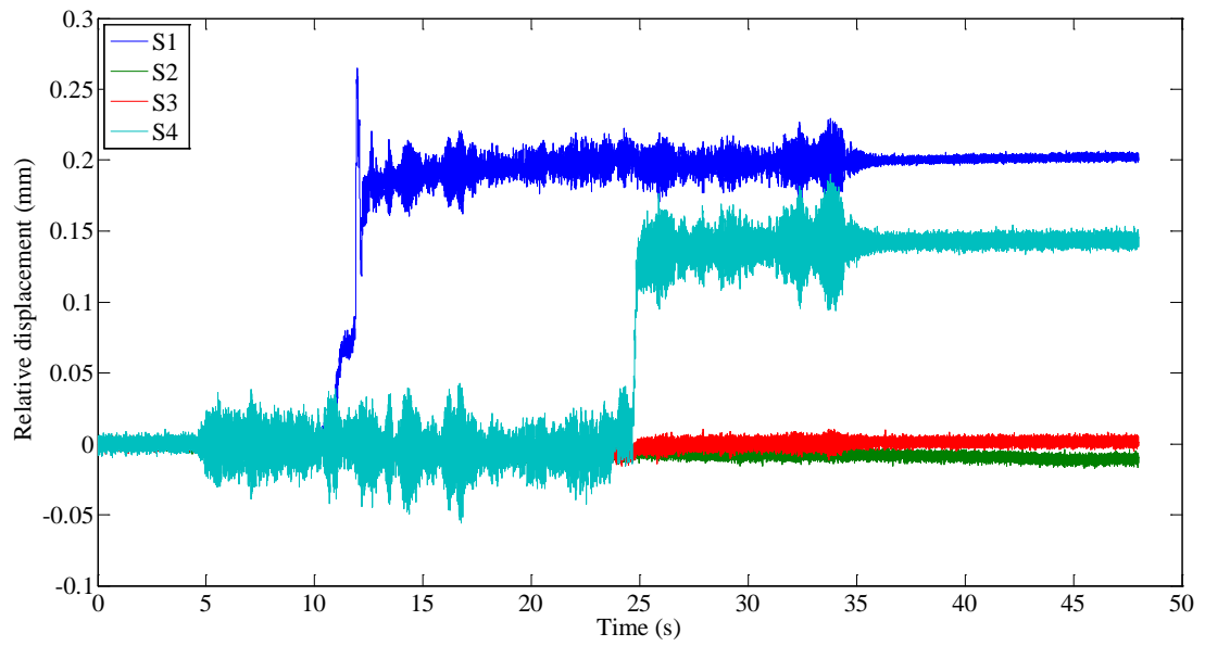
Figure 14 - Online health monitoring with relative displacements under ambient vibrations
