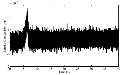
Figure 13 - Study on the sensitivity radius of a relative displacement sensor (S1)
