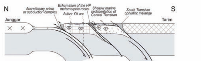
(4) Thrusting related to the closure of the Junggar Ocean (C 3 -P 1 )
