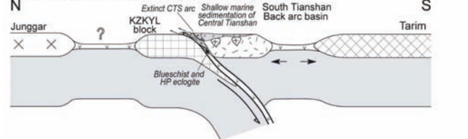
(3) Closure of the South Tianshan back-arc basin and occurrence of arc magmatism in the north margin of Yili-Kazakhstan block (before C 2 )
