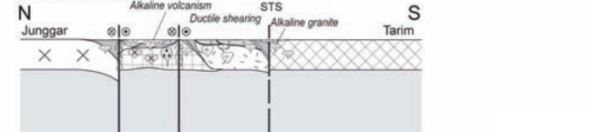
Figure 2. A tentative geodynamic model for the Paleozoic Chinese Tianshan (modified from Wang et al., 2008; Lin et al., 2009)
