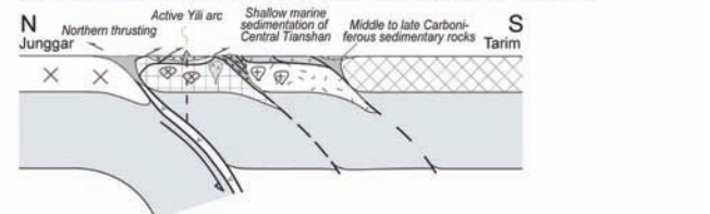
(5) Dextral strike slip (P)
