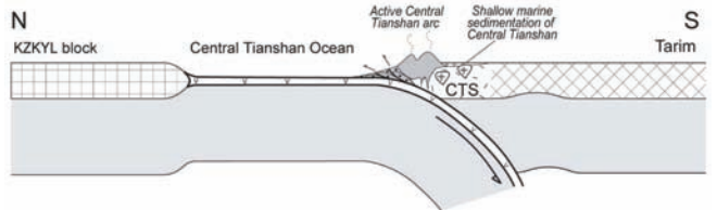
(2) Continental collision, exhumation of HP metamorphism rocks and opening of the South Tianshan back-arc basin (S 2 -C 1 )
