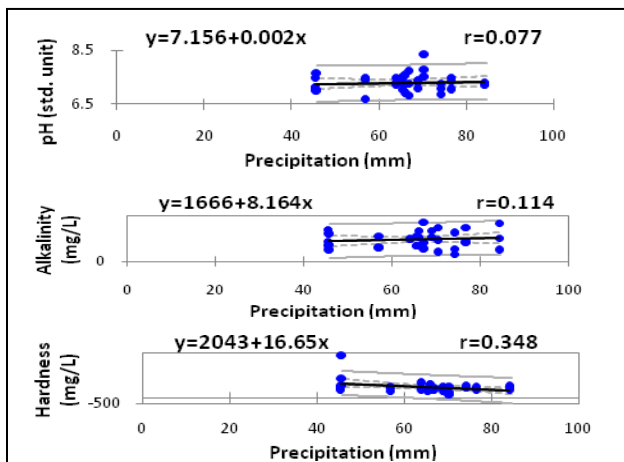
Figure 6 Physical Properties of Leachate Versus Precipitation
