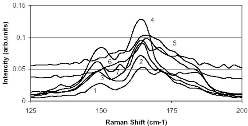
Figure 12. Raman spectra (RBM) at 514nm laser excitation energy (Table 3)
