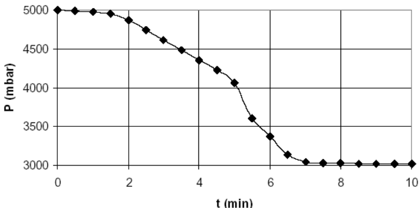
Figure 2. The dependence of pressure drop in the container with non-irradiated CNT samples upon time during container with samples cooling ( P_F = 5035 mbar) (Obolensky et al., 2011b)
