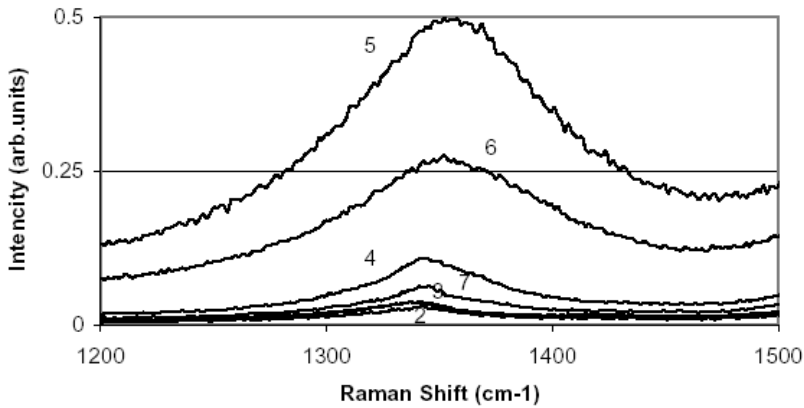
Figure 13. Raman spectra (D band) at 514nm laser excitation energy (Table 3)
