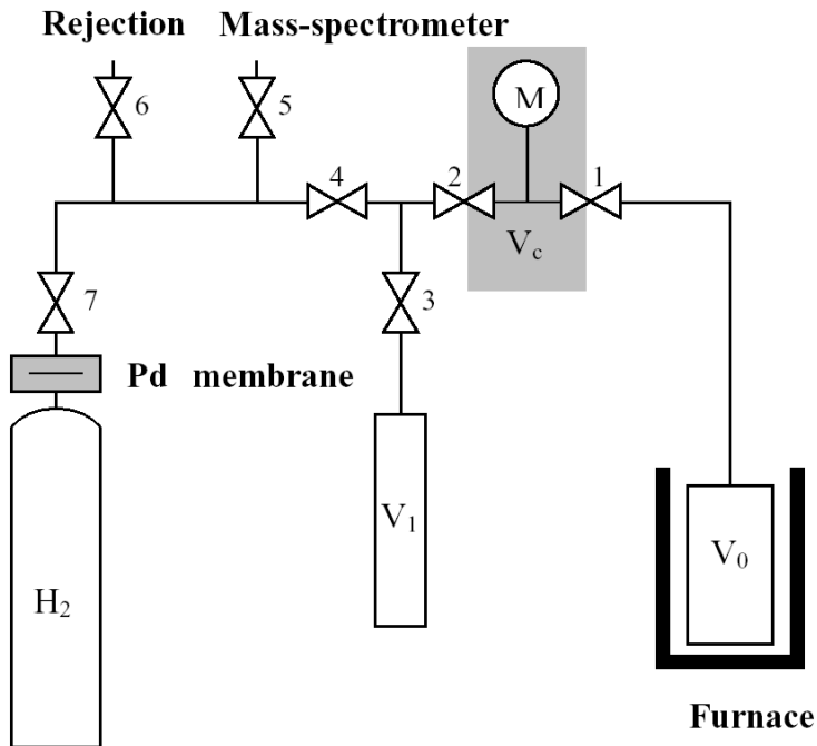
Figure 1. Experimental facility schematics (Obolensky et al., 2011b). V_c – total accurate including manometer and supply pipelines; V_1 – vessel with pure gas; V_0 – ampoule with carbon nanotubes sample; \text{H}_2 – non-purified hydrogen source
