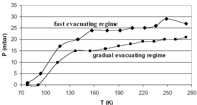
Figure 3. The dependence of pressure in the container with non-irradiated CNT samples upon temperature during container heating for different evacuation rates (Obolensky et al., 2011b)
