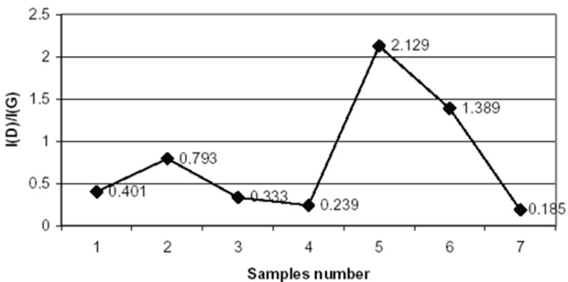
Figure 14. Distribution of the intensity ratio I(D)/I(G) for samples (Table 3)
