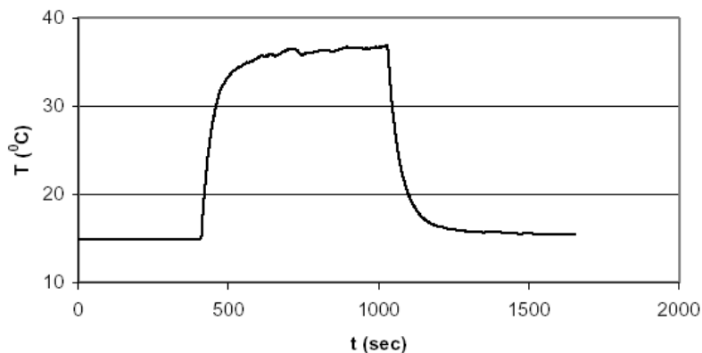
Figure 10. The dependence of samples temperature on the irradiation time (fluence 10^{15}e/cm^2 )
