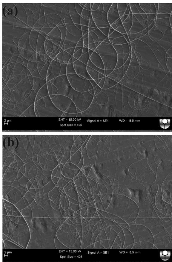
Fig. 8. SEM micrographs of the confirmation experiment for the optimum combination of factors ( A_{60}B_1C_4D_{18} ) using two different needle sizes: (a) 0.514 mm and (b) 0.819 mm. All scale bars represent 2 \mu\text{m} .
