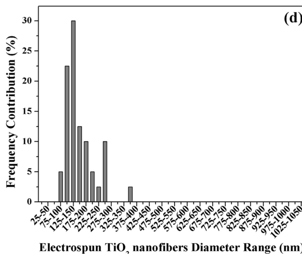
Fig. 4. Frequency contributions to electrospun TiO 2 /PVP nanofibers diameter range in DoE study: (a) T1, (b) T2, (c) T3, (d) T4, (e) T5, (f) T6, (g) T7, (h) T8, and (i) T9.
