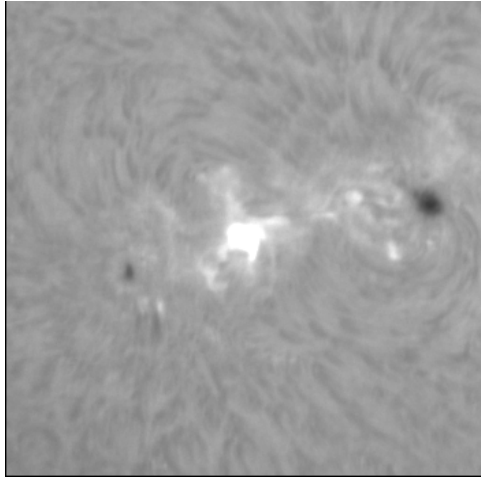
Figure 1. Sample flare image from GONG Big Bear obtained on 2012/07/30 at 15:45:54 UT (location S21.6E28.1). Image is 535 × 535 arcseconds.
