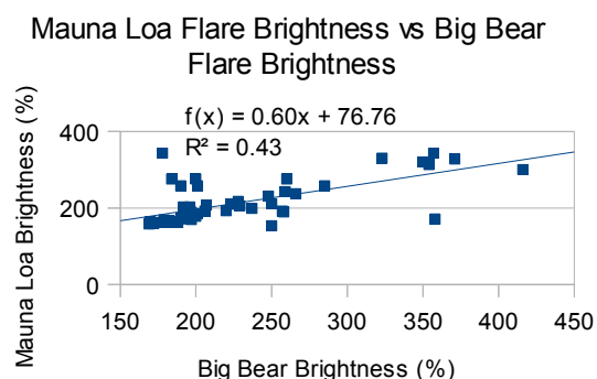
Figure 8. Mauna Loa Flare Brightness vs Big Flare Brightness
