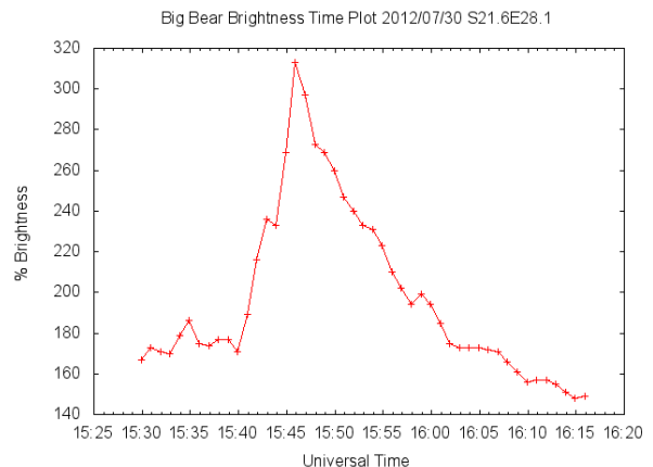
Figure 4. Sample Brightness vs Time Plot from GONG Big Bear.
