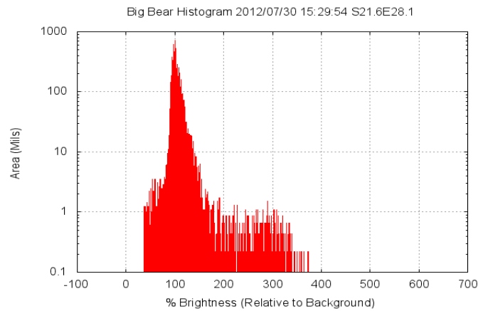
Figure 2. Sample flare histogram from GONG Big Bear.
