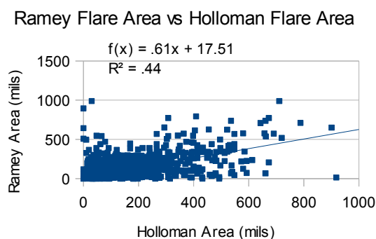
Figure 5. Ramey vs Holloman Flare Area.
