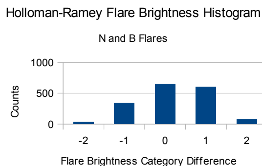
Figure 6. Ramey vs Holloman Flare Brightness. Note that individual bin values are not available in archived data, thus only flare categories were used.
