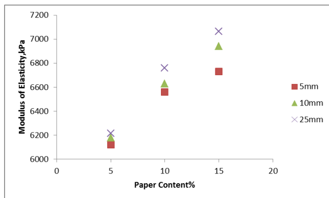
Fig. 4 Effect of paper percentage and length on modulus of elasticity
