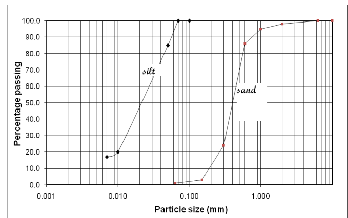
Fig. 1 PSD of used sand (Chegenizadeh and Nikraz,2011)
