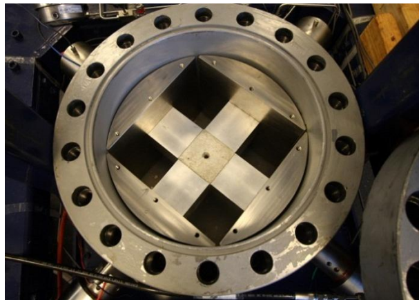
Figure 5. A view of the true triaxial stress cell (TTSC) developed at Curtin Petroleum Engineering (top) and a view of a 100mm sample placed in the cell with a hole drilled at its centre (Rasouli and Evans, 2010).
