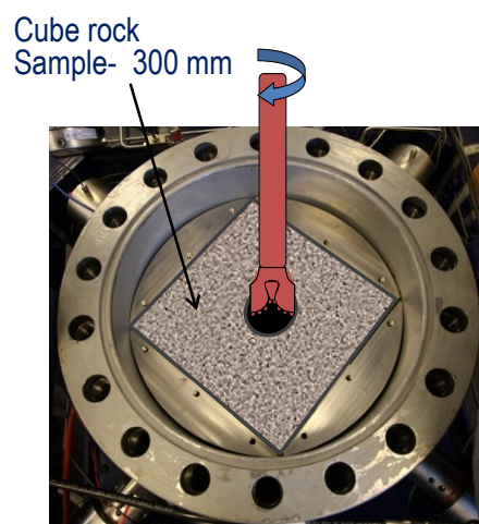
Figure 6. Schematic of drilling through a cubic rock sample subjected to three independent stresses.
