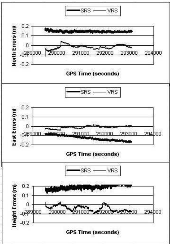
Fig. 5. OLSL station kinematic position accuracy by using the SRS and the VRS methods
