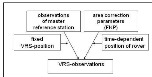
Fig. 1. Generation of the S-VRS data (adapted from [22])
