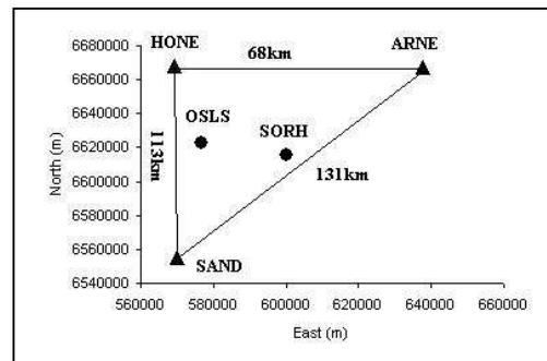
Fig. 3. Norway simulation network
