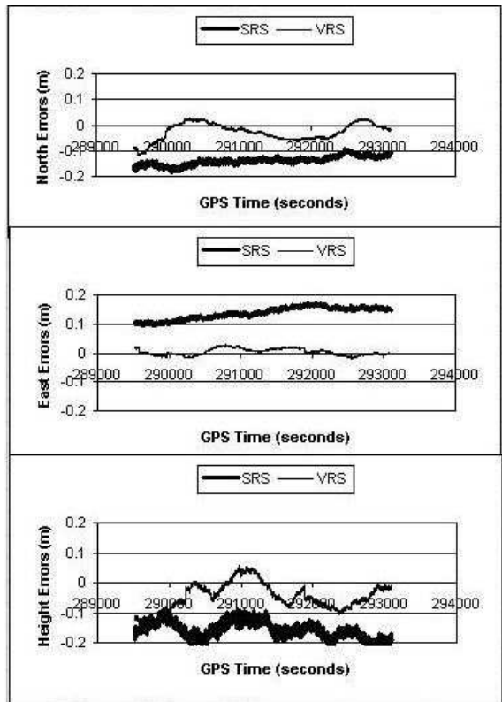
Fig. 4. SORH station kinematic position accuracy by using the SRS and the VRS methods
