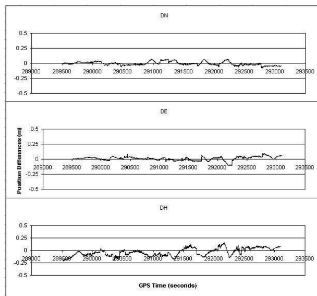
Fig. 8b. Norway airborne GPS kinematic position accuracy by using the MS-VRS method
