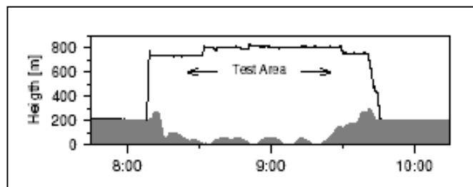
Fig. 7. The height and terrain profile of the test flight (from [14])
