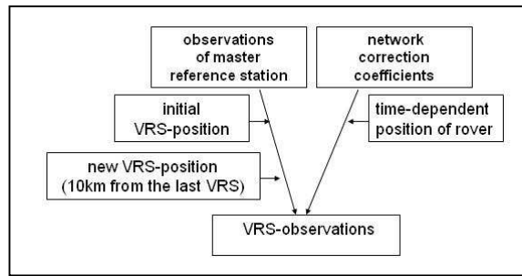
Fig. 2. Generation of the MS-VRS data
