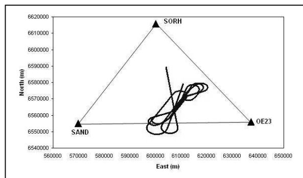
Fig. 6. Flight trajectory and the reference stations network of the selected test data
