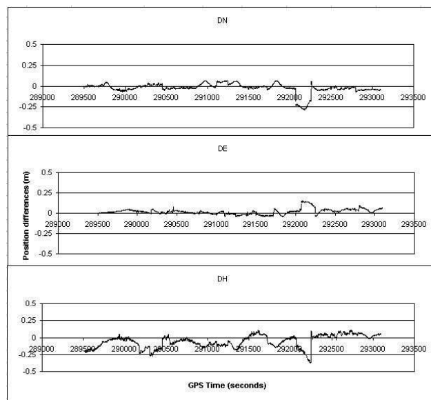
Fig. 8a. Norway airborne GPS kinematic position accuracy by using the S-VRS method
