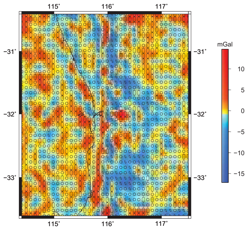
Fig. 8 Elliptical kernels attributed to each observation (gravity) point used to construct the non-stationary auto-covariance matrix \mathbf{C}_{\varepsilon_{\Delta g}, \varepsilon_{\Delta g}} . The underlying image shows the residual anomalies referenced to EGM2008 [units in mGal; Mercator projection]
