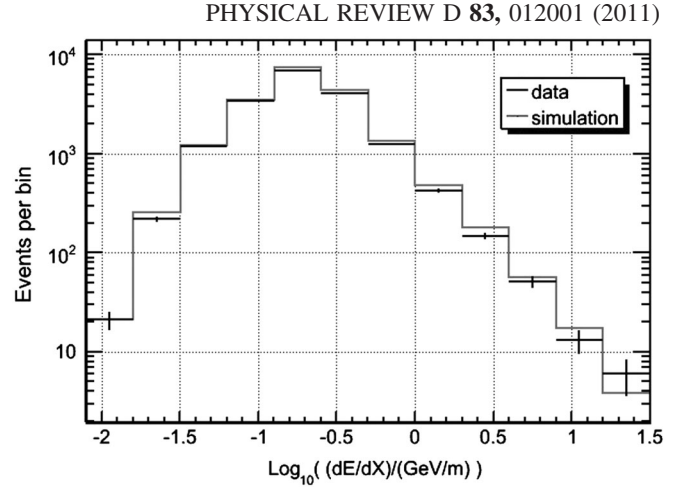
FIG. 13. Distributions of the dE/dX observable, for data and for simulation. The additional cut at zenith angle of 97^\circ has been applied. Error bars for data are statistical only.
