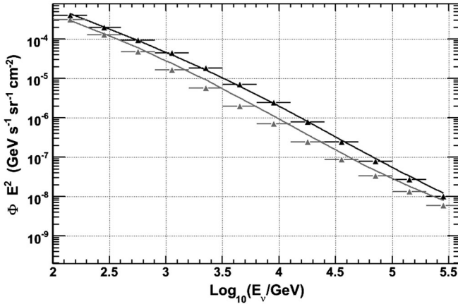
FIG. 20. Comparison of unfolded energy spectra for different zenith ranges. Separate unfoldings were performed for the zenith range 97^\circ\text{--}124^\circ (black) and the zenith range 124^\circ\text{--}180^\circ (gray). The unfolded results for each region (horizontal lines) and the predicted spectrum corresponding to each region (curves) are shown. Uncertainties for these results are not shown.
