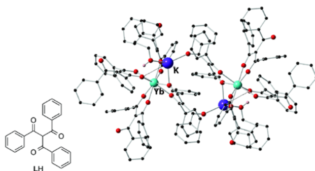
Figure 1. Ligand LH and X-ray crystal structure of [\text{Yb}(\text{K-HOEt})(\text{L})_4]_2 . H atoms, aside from ethanol OH, are omitted for clarity.
