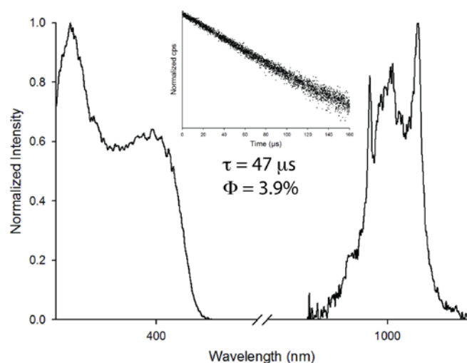
Figure 2. Excitation and emission spectra of [\text{Yb}(\text{K-HOEt})(\text{L})_4]_2 . The emission spectrum was recorded upon excitation at \lambda_{\text{ex}} = 350 nm. Inset: excited state decay measured by monitoring the emission at \lambda_{\text{em}} = 1,035 nm.
