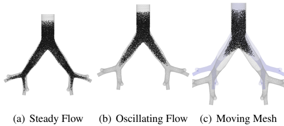
Figure 6: Particle ingress after 0.25s
