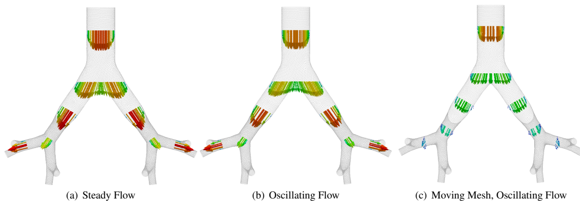
Figure 4: Velocity at various cross-sections at maximum inspiration.
