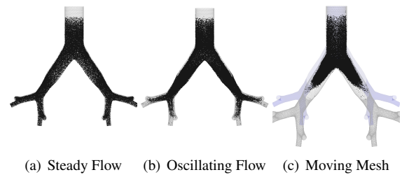
Figure 7: Particle ingress after 5s
