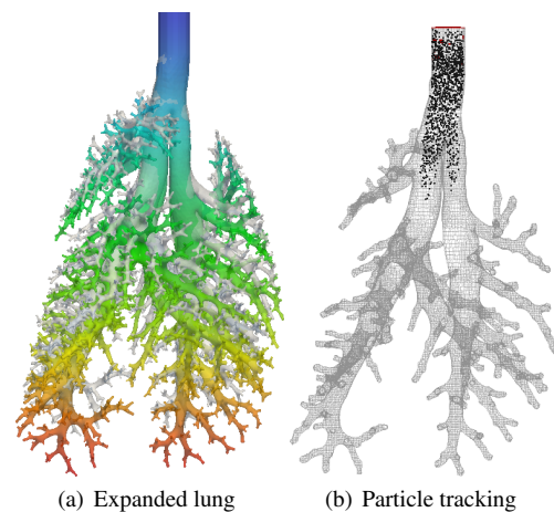
Figure 8: Imposed mesh motion, and particle tracking inside the lung of high resolution Sprague-Dawley rat model. In (a) Colours indicate maximum displacement, and the grey boundary the undeformed mesh, in (b) particle locations are indicated in black.
