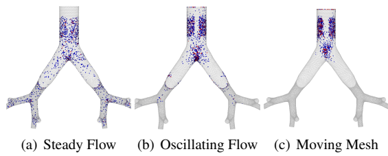
Figure 5: Particle deposition locations after 5s
