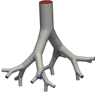
Figure 1: Mesh and boundary locations
