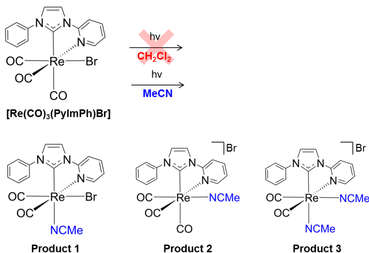
Figure 1: Structures of [Re(CO)_3(PyImPh)Br] and its photoreaction products upon irradiation by UV light of a solution in MeCN of [Re(CO)_3(PyImPh)Br] .
