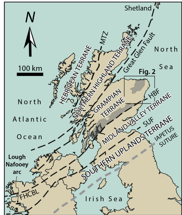
Figure 1. Terrane map of the British Isles. The Buchan Block, part of the wider Grampian Terrane, is located within the box (see Fig. 2). The darker shading shows the outcrop of Southern Highland Group rocks in Scotland. HBF = Highland Boundary Fault; FHCBL = Fair Head–Clew Bay line; SUF = Southern Uplands Fault. The location of the Lough Nafuoey arc and the proposed position of the Iapetus suture are indicated.
