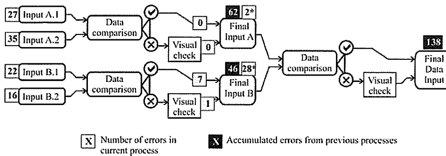
Figure 2: Identified quantity of input errors
