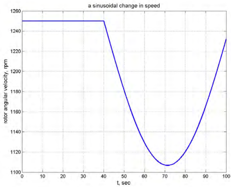
Figure 4 A change in the machine shaft speed occurring at t = 40 sec
