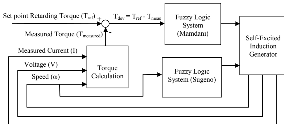
Figure 2 Control scheme of a self-excited induction generator using two fuzzy logic systems
