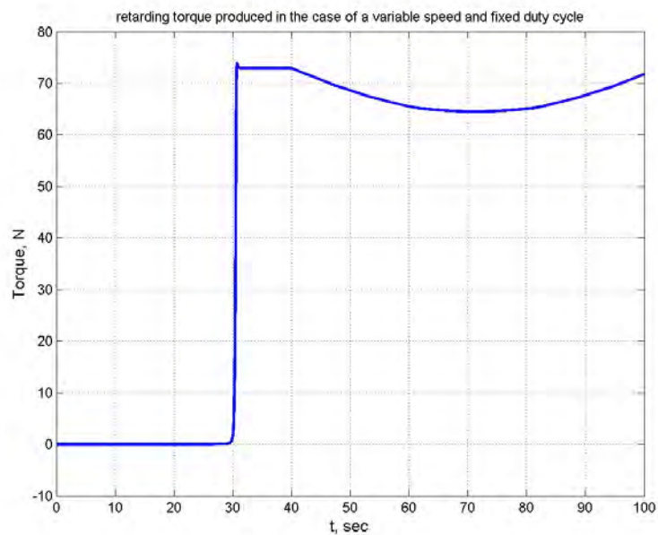
Figure 5 Retarding torque changes as a result of the change in speed
