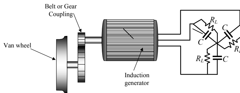
Figure 1 Electrical braking system using an induction generator (adapted from [2])
