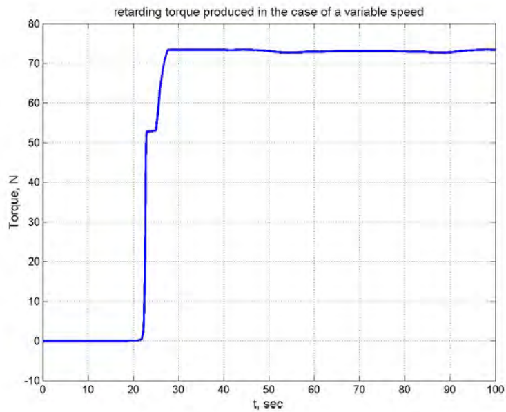
Figure 7 Torque output is kept fairly constant after the initial voltage build up
