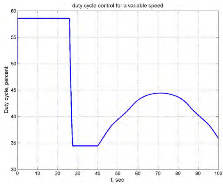
Figure 6 The fuzzy logic controller adjusts the duty cycle to maintain a constant torque
