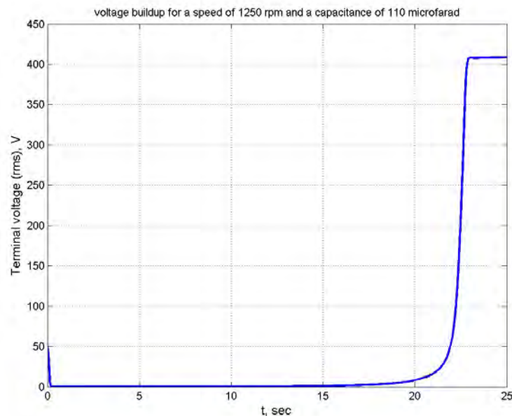
Figure 3 The initial voltage build up, with a charged capacitor and at a constant speed
