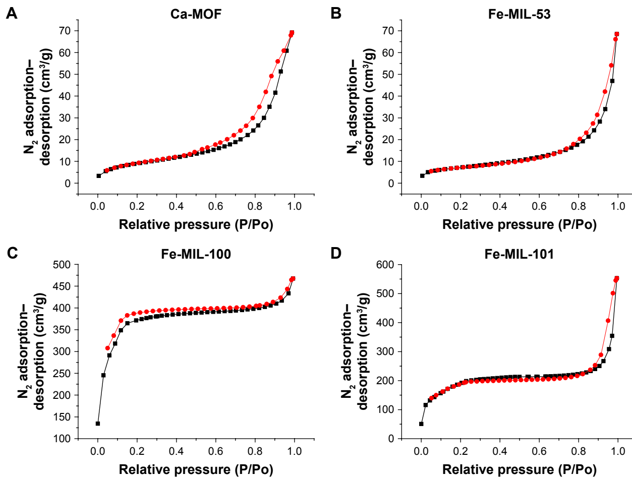
Figure S2 N 2 adsorption-desorption behavior of Ca-MOF (A), Fe-MIL-53 (B), Fe-MIL-100 (C), and Fe-MIL-101 (D). Abbreviation: MOF, metal organic framework.
