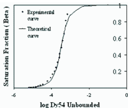
Fig. 9. Zimm-Bragg isotherm for ALG-DY54 (HCl) system. (with permission of J. Mex. Chem. Soc.)
