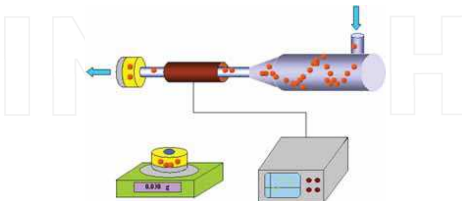
Fig. 5. Measurement of the q/m -values with the inductive cylindrical probe.
