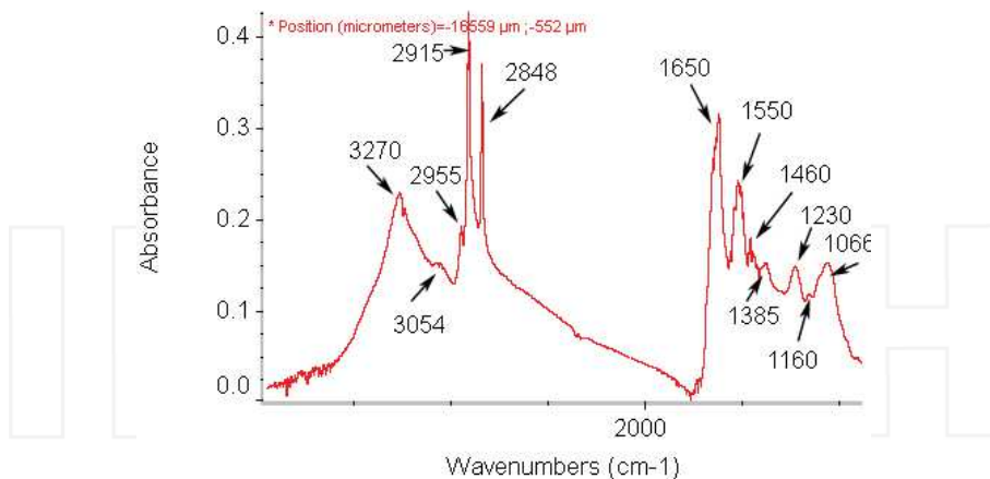
Fig. 2. Typical spectrum of sorghum germ tissue within cellular and sub-cellular dimensions showing broad N-H and O-H stretching band at ca. 3270 \text{ cm}^{-1} , \text{CH}_2 and \text{CH}_3 anti-symmetric and symmetric stretching bands at the region of ca. 2990\text{-}2780 \text{ cm}^{-1} , amide I and II bands at ca. 1650 \text{ cm}^{-1} and 1550 \text{ cm}^{-1} , respectively and cellulosic compound bands region of ca. 1200\text{-}800 \text{ cm}^{-1} , using ultra-spatially resolved synchrotron-based FTIR microspectroscopy at National Synchrotron Light Source, Brookhaven National Lab (U.S. Dept of Energy, NY).
