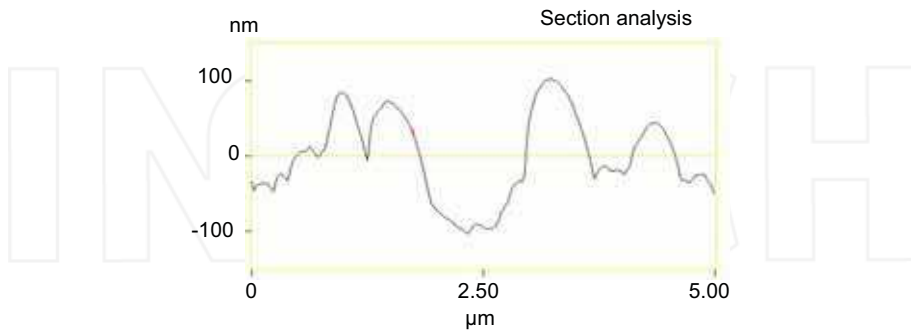
Fig. 14a. AFM roughness profile for raw C17 cotton fibre
