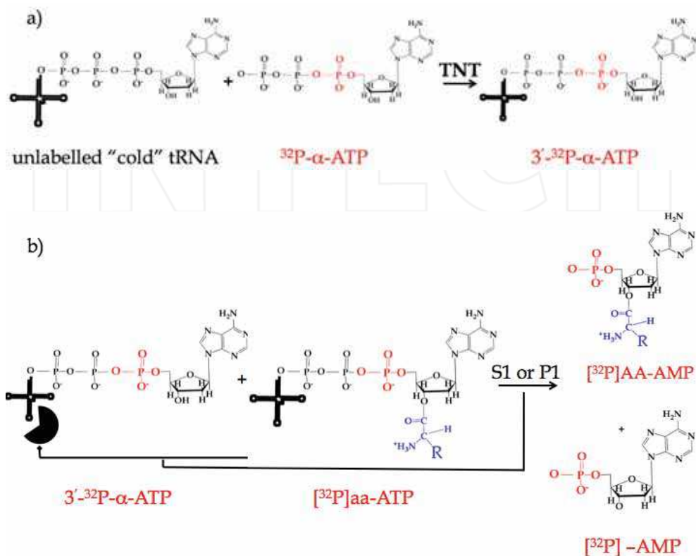
Fig. 8. Panel a) Schematic of the 3'- 32 P labelling procedure using the repair/ processing enzyme terminal nucleotidyl transferase (TNT). Panel b) displays the hydrolysis products following enzymatic digestion with either nuclease S1 or P1.
