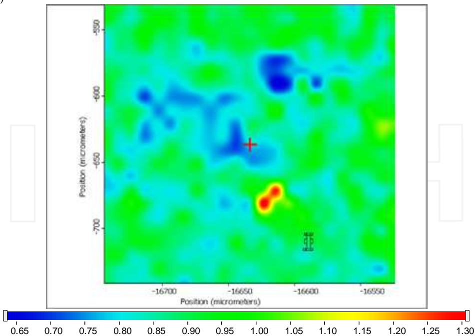
Peak height ratio ca. 1657/1628 cm -1 (Chemical image)
