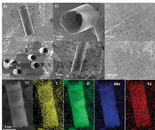
Fig. 1 Scanning electron microscopy (SEM) and energy dispersive X-ray (EDX) mapping analysis of the \text{erGO/FeO}_x\text{-MnO}_2 micromotors: (A) a lying microtube, (B) an upright microtube, (C) a number of microtubes, (D) an array of microtubes, (E) a lying microrod, (F) a number of microrods, and (G) EDX mapping analysis of a microtube.
