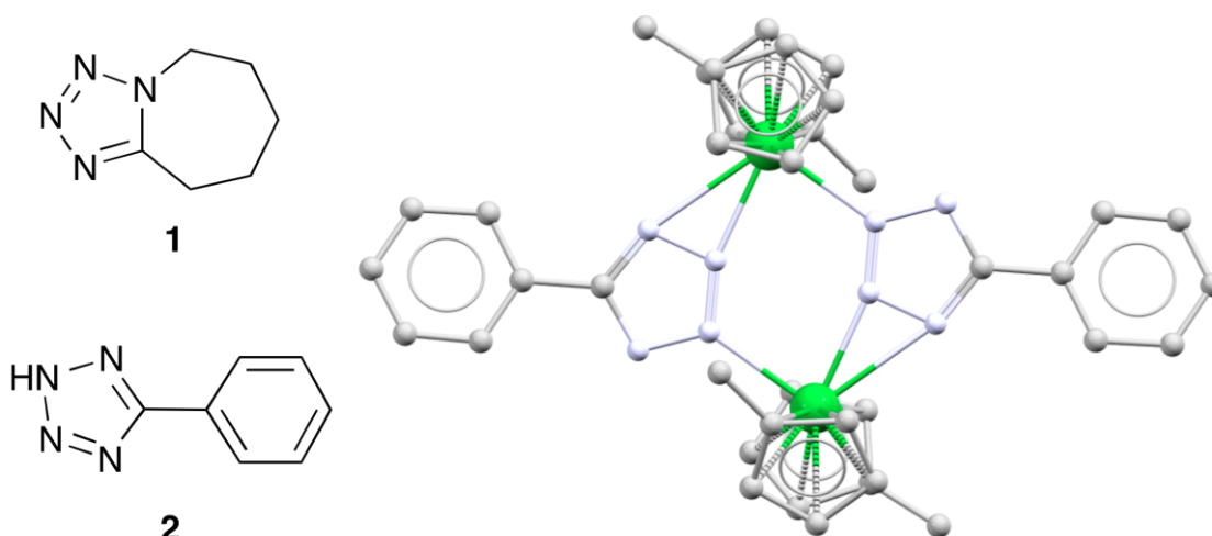
Figure 1. Tetrazole ligands used in structurally characterised organometallic lanthanoid complexes: 1 , [17] 2 , and a representation of the molecular structure of [(C_5H_4Me)_2Yb(\mu - \eta^1 : \eta^2 - (2-H))] _2 emphasising the tetrazole ligand bridging mode. [18]
