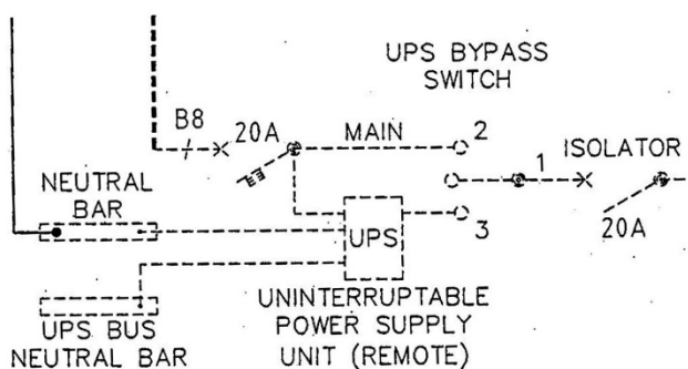
Figure 5. Circuit breaker rating on SIP-LG37 and SIP-L016
