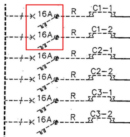
(a) Circuit breaker rating on SIP-LG37
