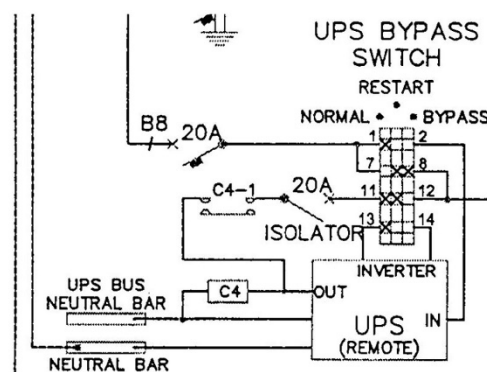
Figure 5. Circuit breaker rating on SIP-LG37 and SIP-L016
