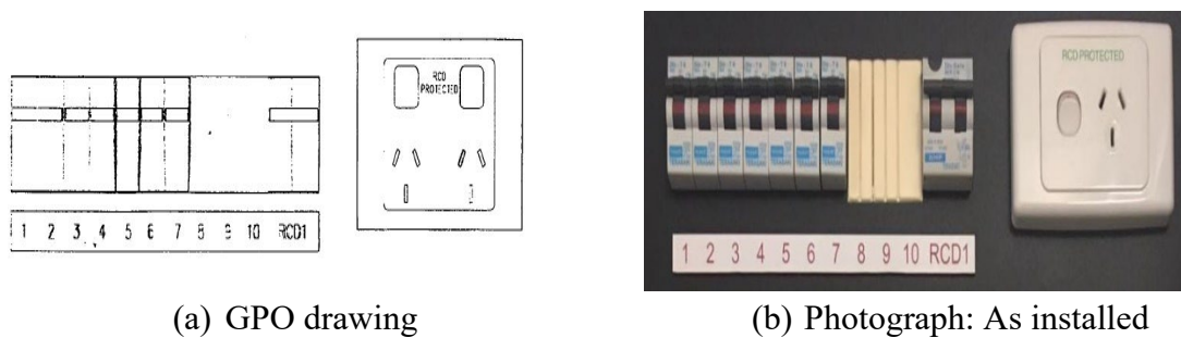
Figure 7. GPO: ‘As-built’ versus ‘as-installed’
