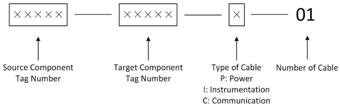
Figure 4. Example of cable numbering
