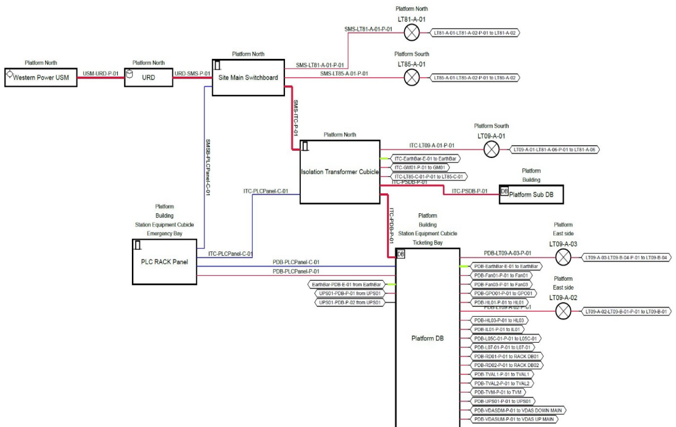
Figure 10. SIM block connection
