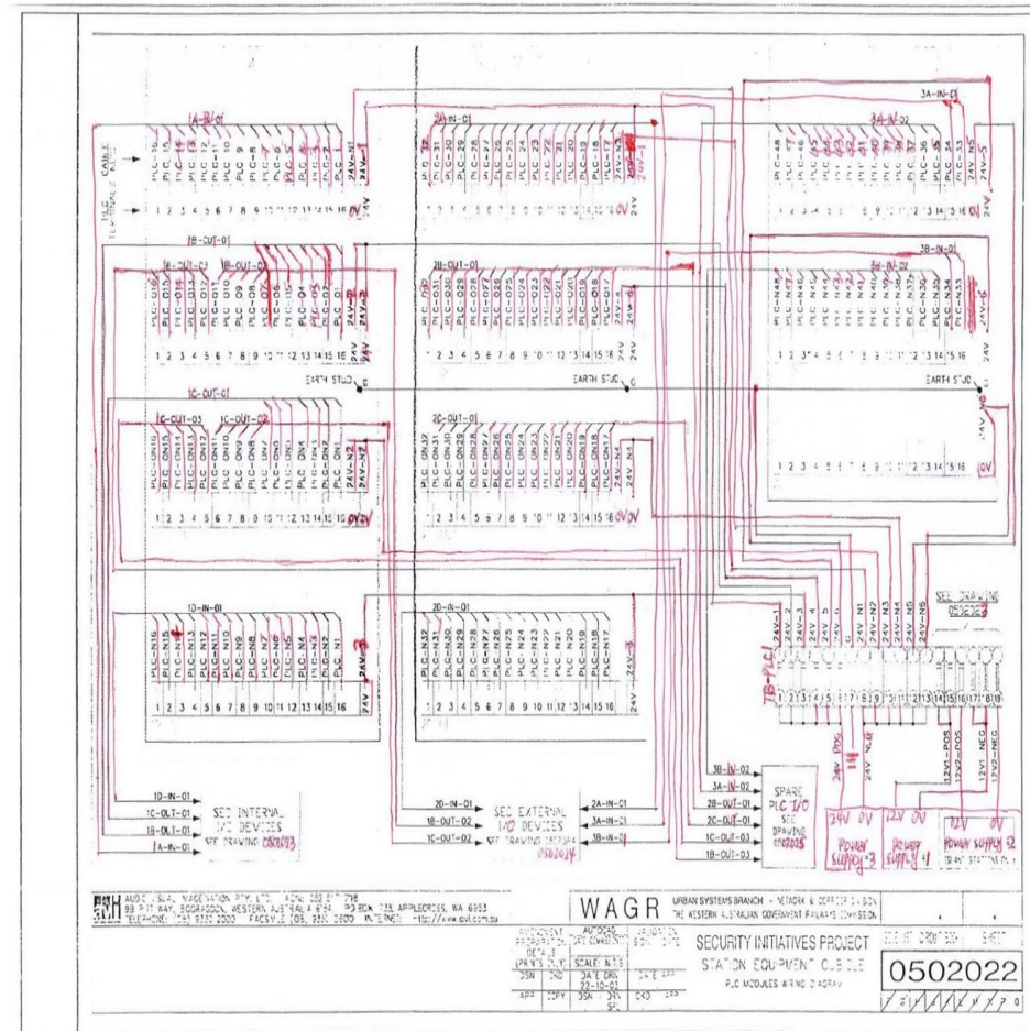
(a) Redrawn 'as-built'
