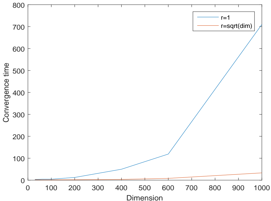
Figure 4: Convergence time when dimension increases
