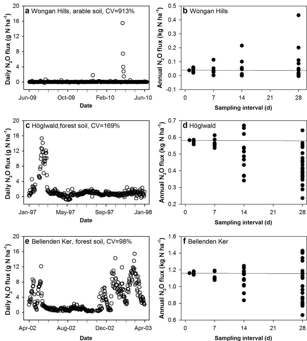
Figure 1. Daily N_2O fluxes and the influence of sampling frequency on annual N_2O fluxes. The daily N_2O flux (a,c,e) for the three data sets shown have varying coefficients of variation (CV), which influences the effect of sampling frequency on annual N_2O fluxes (b,d,f). See Table 4 for description of sampling intervals.
