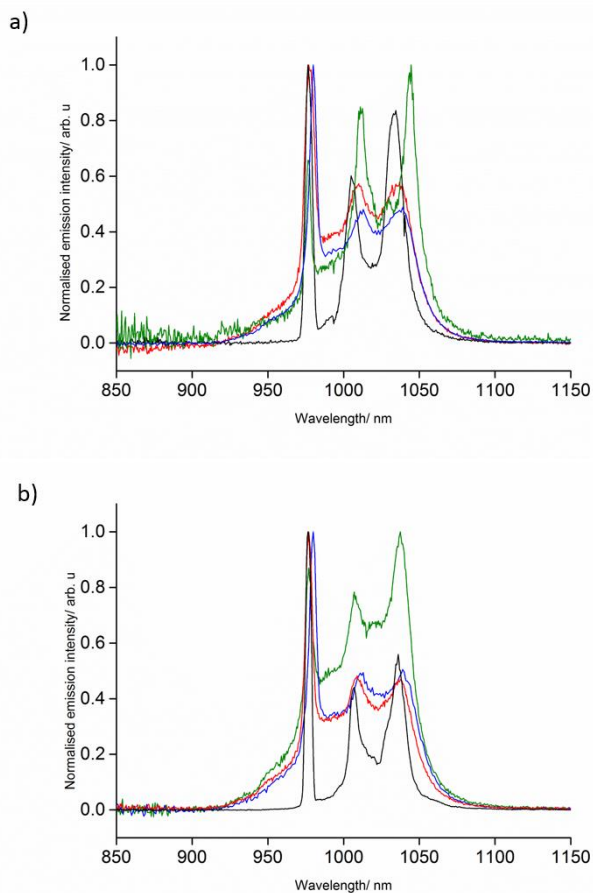
Figure 4.- Normalised emission plots for a) [\text{Yb}(\text{phen})(\text{tbm})_3] and b) [\text{Yb}(\text{phen})(\text{dbm})_3] in solid state (green trace), DCM solution(10-5M) (red trace), 77K (back trace) and PMMA (blue trace), with excitation wavelength at 350nm.
