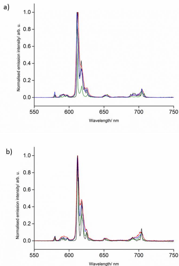
Figure 3 - Normalised emission plots for a) [\text{Eu}(\text{phen})(\text{tbm})_3] and b) [\text{Eu}(\text{phen})(\text{dbm})_3] in solid state (green trace), DCM solution (10-M) (red trace), 77 K (black trace) and PMMA (blue trace), with excitation wavelength at 350 nm.
