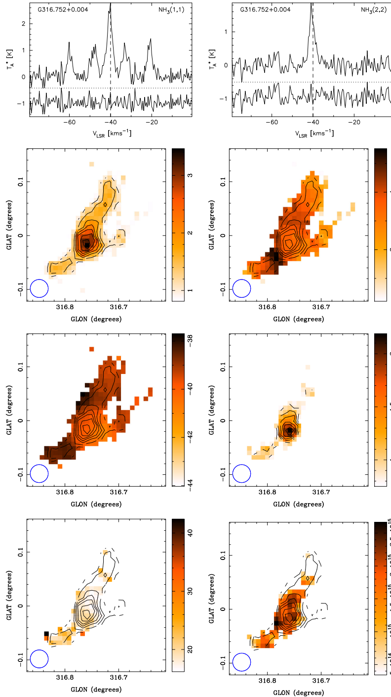
Figure 2. Spatially resolved gas properties output from the automated spectral-line fitting routine, for example source G316.752 + 0.004 – 38.2 (see Paper II for the naming definition). \text{NH}_3 (1,1) [top left] and \text{NH}_3 (2,2) [top right] spectra from the pixel with peak \text{NH}_3 (1,1) emission, with residuals from the fit displayed underneath. The vertical dashed lines show the \text{NH}_3 (1,1) V_{\text{LSR}} . The left-hand panel of the second row shows the brightness temperature (in K) of the \text{NH}_3 (1,1) emission overlaid with contours in 10 per cent steps of the peak value, from 90 per cent down. The right-hand panel of the second row and left-hand panel of the third row show the velocity dispersion and V_{\text{LSR}} (in \text{km s}^{-1} ) of the \text{NH}_3 (1,1) emission determined from the fit to each pixel. The contours for these two plots show the same \text{NH}_3 (1,1) brightness temperature contours as the left-hand panel of the second row. The right panel on the third row shows the brightness temperature (in K) of \text{NH}_3 (2,2) emission overlaid with contours in 10 per cent steps of the peak value, from 90 per cent down. The bottom left and right panels show the kinetic temperature (in K) and total \text{NH}_3 column density (in \text{cm}^{-2} ) maps, respectively. The contours for these two plots show the same \text{NH}_3 (2,2) brightness temperature contours as the right-hand panel of the third row. The primary beam is shown in the bottom left corner of each image.
