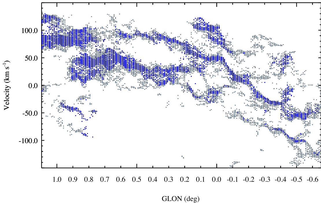
Figure 28. Comparison of the Henshaw et al. (2016) fits to the Jones et al. (2012) Mopra 3mm HNC emission (grey) and the HOPS \text{NH}_3(1,1) emission (blue). In the overlapping spatial coverage range between the two data sets (longitudes of -0.7 \lesssim l \lesssim 1^\circ ) the \text{NH}_3 PPV structure closely matches that of the HNC, despite the factor \sim 4 lower angular resolution. This gives confidence that the source fits to these high-density tracers are robustly tracing the global gas kinematics.
