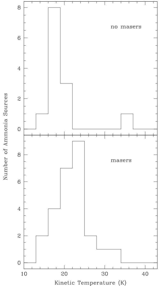
Figure 8. Distributions of kinetic temperatures for \text{NH}_3 sources. The distributions are shown for \text{NH}_3 clumps with no known maser association (top) and associations either water and/or methanol masers (bottom). The top distribution shows typically lower kinetic temperatures.
