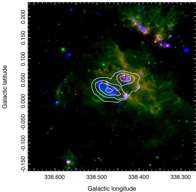
Figure 17. Three-colour images of YMC progenitor gas cloud candidate G338.464+0.034 [red, HiGAL 70\ \mu\text{m} (Molinari et al. 2010); green, 8\ \mu\text{m} GLIMPSE (Churchwell et al. 2009); blue, ATLASGAL 850\ \mu\text{m} emission (Schuller et al. 2009)]. Crosses are methanol masers (Caswell et al. 2010, 2011) and plus symbols are HOPS water masers (Walsh et al. 2011, 2014). White contours show the \text{NH}_3 (1,1) integrated intensity emission.
