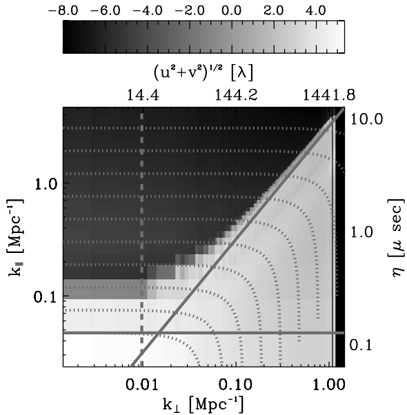
Figure 6. Same as Figure 5 but for an extended Blackman–Nuttall bandpass window. The spillover into the EoR window around (k_{\perp}, k_{\parallel}) \simeq (0.01, 0.2) \text{ Mpc}^{-1} is \sim 10^{-5} \text{ K}^2 \text{Hz}^2 .
