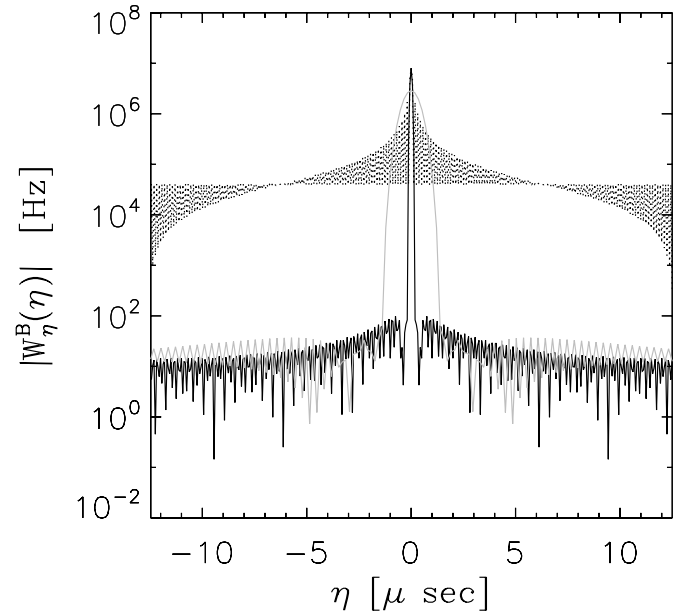
Figure 4. Amplitude of the responses of the bandpass window functions of Figure 3 shown vs. \eta , the instrumental delay. Line styles are identical to those in Figure 3. The responses of rectangular and extended Blackman–Nuttall bandpass windows are almost identical in sensitivity and resolution along \eta , while the standard Blackman–Nuttall window is poorer in resolution and \approx 2.76 times lesser in sensitivity.
