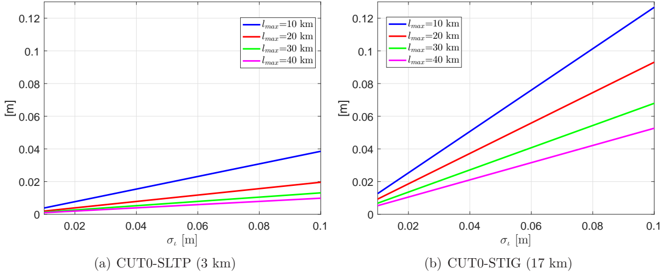
Fig. 7. Standard deviations of the ionospheric spatial constraints (Eq. A.3) for (a) baseline CUT0-SLTP of around 3 km and (b) baseline CUT0-STIG of around 17 km. The mean elevation angle \bar{e}^s (Eq. A.3) was assumed to be 50 degrees
