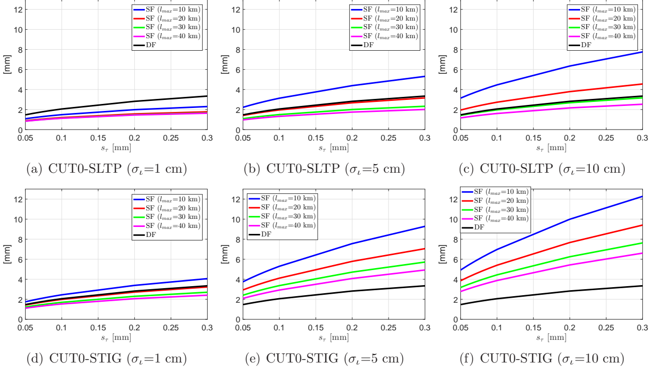
Fig. 8. Average formal standard deviations of the rZWDs for (a, b, c) baseline CUT0-SLTP of around 3 km and (d, e, f) baseline CUT0-STIG of around 17 km. The parameter \sigma_l (Eq. A.3) was set to be (a, d) 1 cm, (b, e) 5 cm and (c, f) 10 cm, respectively. Partial ambiguity resolution was enabled with a pre-defined success rate of 99.9%. For the SF network A and the DF network B, ionosphere-weighted and -float models were applied in the processing, respectively
