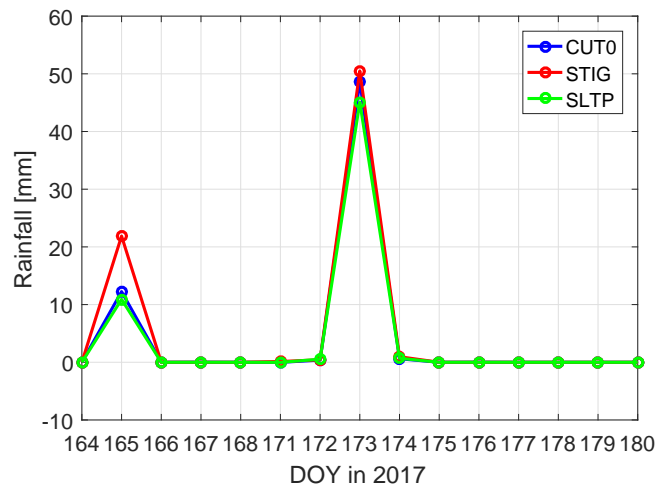
Fig. 2. Interpolated daily rainfall amounts for stations CUT0, STIG and SLTP in 15 days of June 2017. DOY is short for day of year
