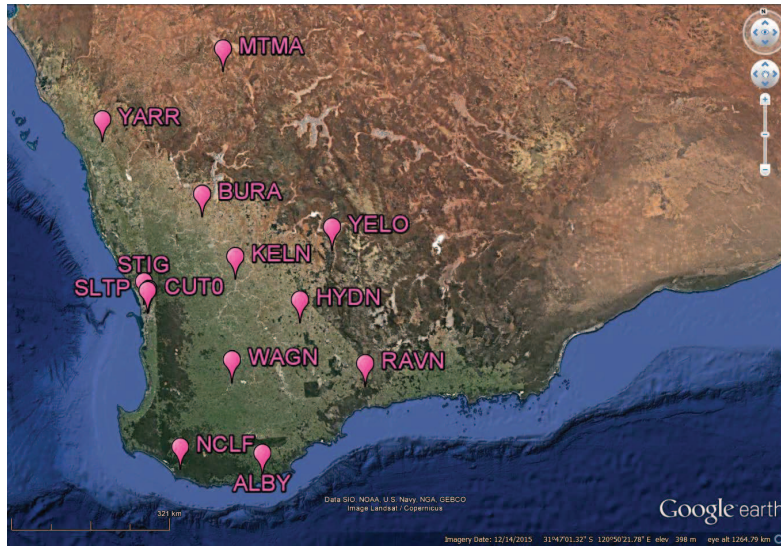
Fig. 4. DF Network B in Western Australia with the largest inter-station distance of around 757 km. Map data: Google, Data SIO, NOAA, U.S. Navy. NGA. GEBCO, Image Landsat/Copernicus (Google Earth 2018b)
