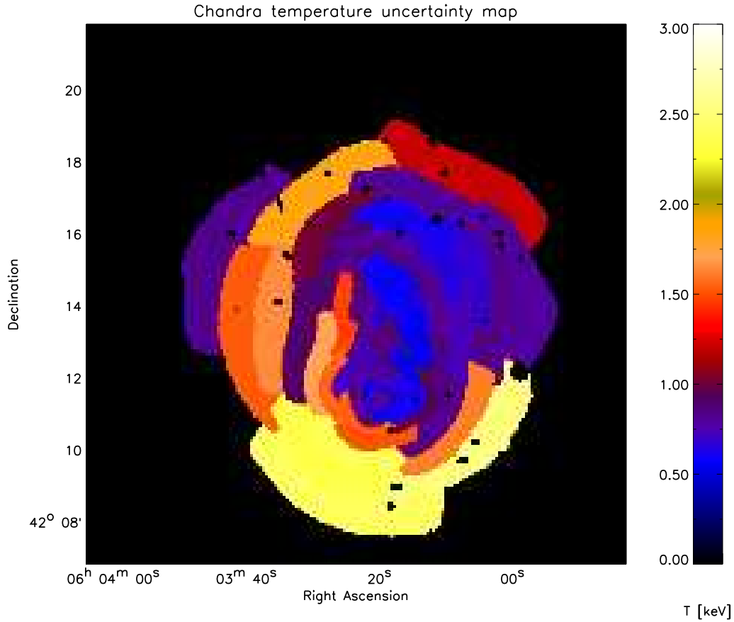
FIG. 17.— Temperature uncertainty map corresponding to Figure 11. The average of the upper and lower 1\sigma temperature errors is shown.
