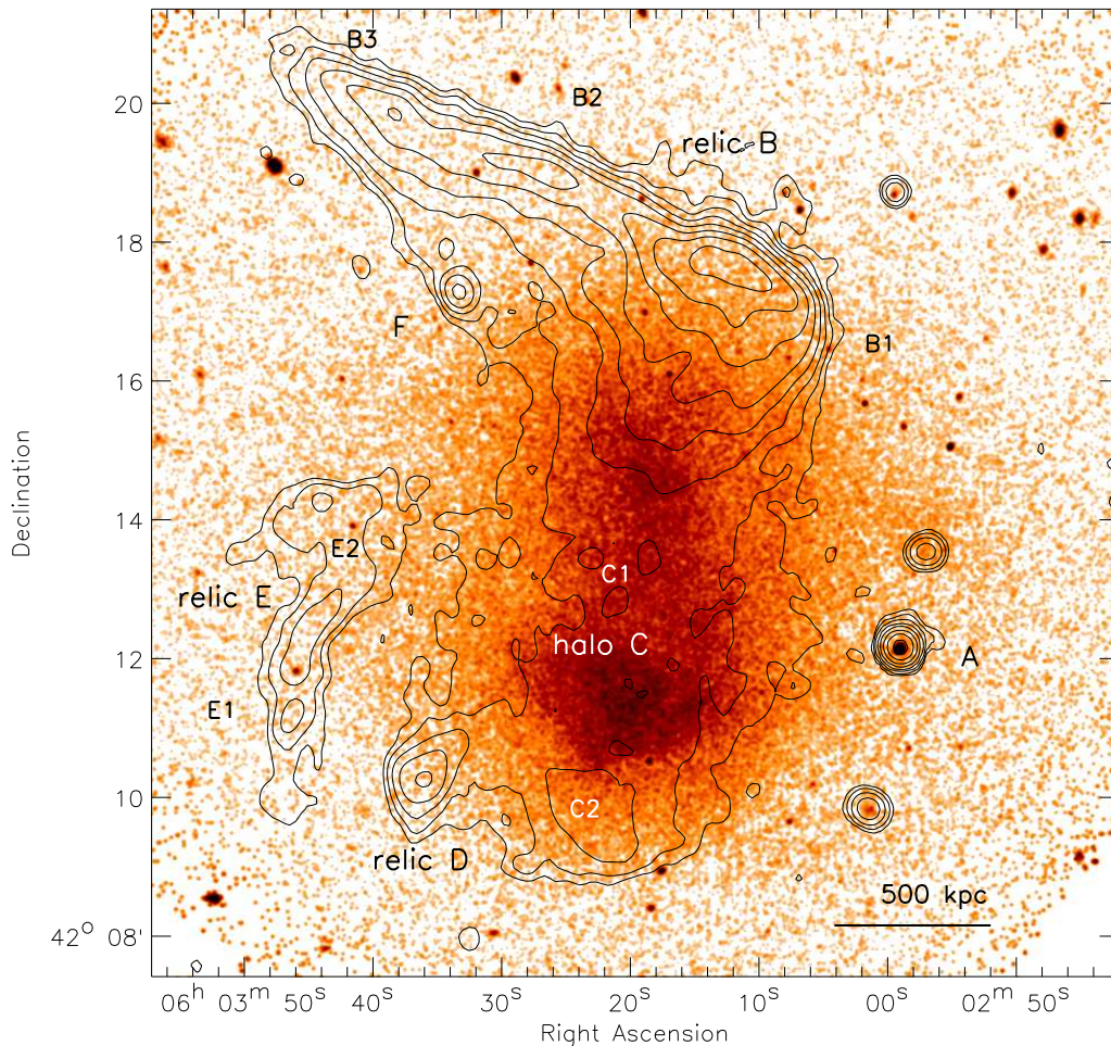
FIG. 9.— Chandra ACIS-I 0.5–2.0 keV image (bin=2) of the Toothbrush cluster. The image is smoothed with a Gaussian with a FWHM of 3'' . Radio contours from the LOFAR image with a resolution of 17.7'' (right panel Figure 3) are overlaid. Radio sources are labelled as in Figure 1. The X-ray image shows two main concentrations, aligned N-S. The southern structure is better defined and has a bullet-like shape (see also Figure 12).
