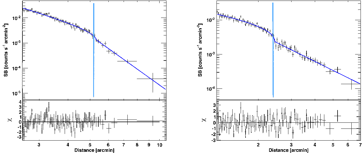
FIG. 13.— Left: X-ray surface brightness profile across the bright part (B1) of the northern Toothbrush relic: Right: X-ray surface brightness profile in the southern sector. The blue lines show the best-fitting broken power-law density model (Eq. 1) and the vertical line the outer boundary of the radio relic or halo emission.
