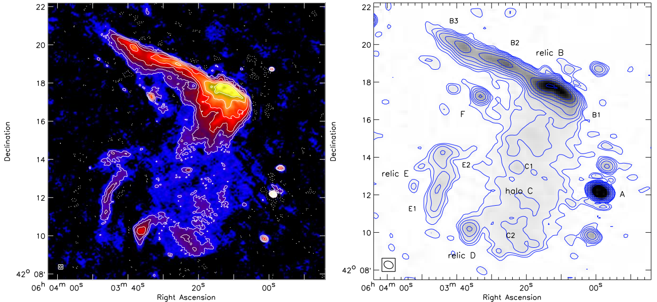
FIG. 1.— Left: LOFAR HBA 120–181 MHz image. The beam size is 8.0'' \times 6.5'' as indicated in the bottom left corner. Contour levels are drawn at [1, 2, 4, 8, \dots] \times 4\sigma_{\text{rms}} , with \sigma_{\text{rms}} = 93 \mu\text{Jy beam}^{-1} . Negative -3\sigma_{\text{rms}} contours are shown with dotted lines. Right: D-array VLA 1–2 GHz image with various sources labelled, following van Weeren et al. (2012a). Some of the sources are further subdivided into numbered components, e.g., relic E is divided into E1 and E2. The beam size is 31'' \times 24'' . Contour levels are drawn at the same levels as in the left panel, but with \sigma_{\text{rms}} = 35 \mu\text{Jy beam}^{-1} .
