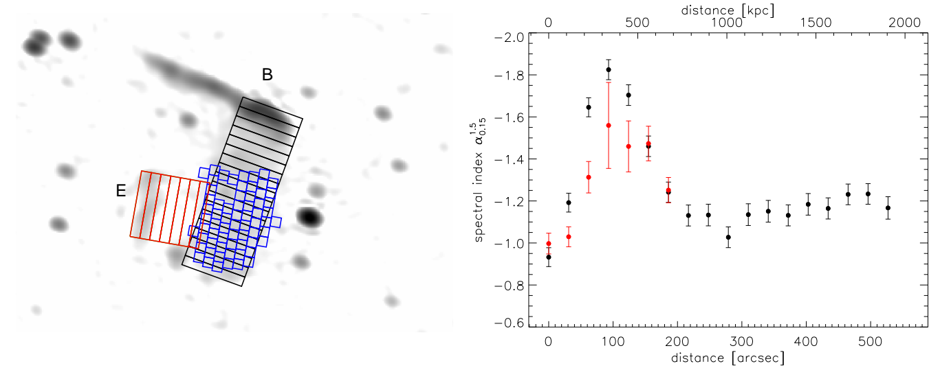
FIG. 8.— Left: Regions where spectral indices were extracted are shown on top of the VLA 1–2 GHz image. The spectral indices for the red and black regions are shown in the left right panel. The spectra for the blue regions are shown in Figure 16. We excluded the regions affected by a compact source located at RA 06^{\text{h}}03^{\text{m}}23^{\text{s}} , Dec 42^{\circ}13'26'' . Right: The spectral index between 0.15 and 1.5 GHz across the E radio relic is shown in red (from east to west). The spectral index across relic B1 and the radio halo, from north to south, is shown in black. The regions have a width of 31'' .
