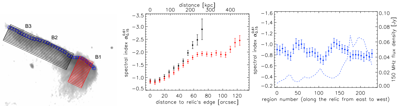
FIG. 6.— Left: Regions where the spectral indices were extracted (displayed in the middle and right panel) on top of a HBA 150 MHz image (used to make Figure 5). Middle: The spectral index between 150 and 610 MHz across relic B1, from north to south, is shown with red points. The black points cover the spectral index for the B2 and B3 part of the relic. The regions have a width of 6.5'' . Right: The blue points trace the spectral index along the northern edge of relic B, with the distance increasing from east to west. The blue regions have sizes of 12'' . The dashed blue line traces the LOFAR 150 MHz flux density along the relic, corresponding to the spectral indices shown in the same color.
