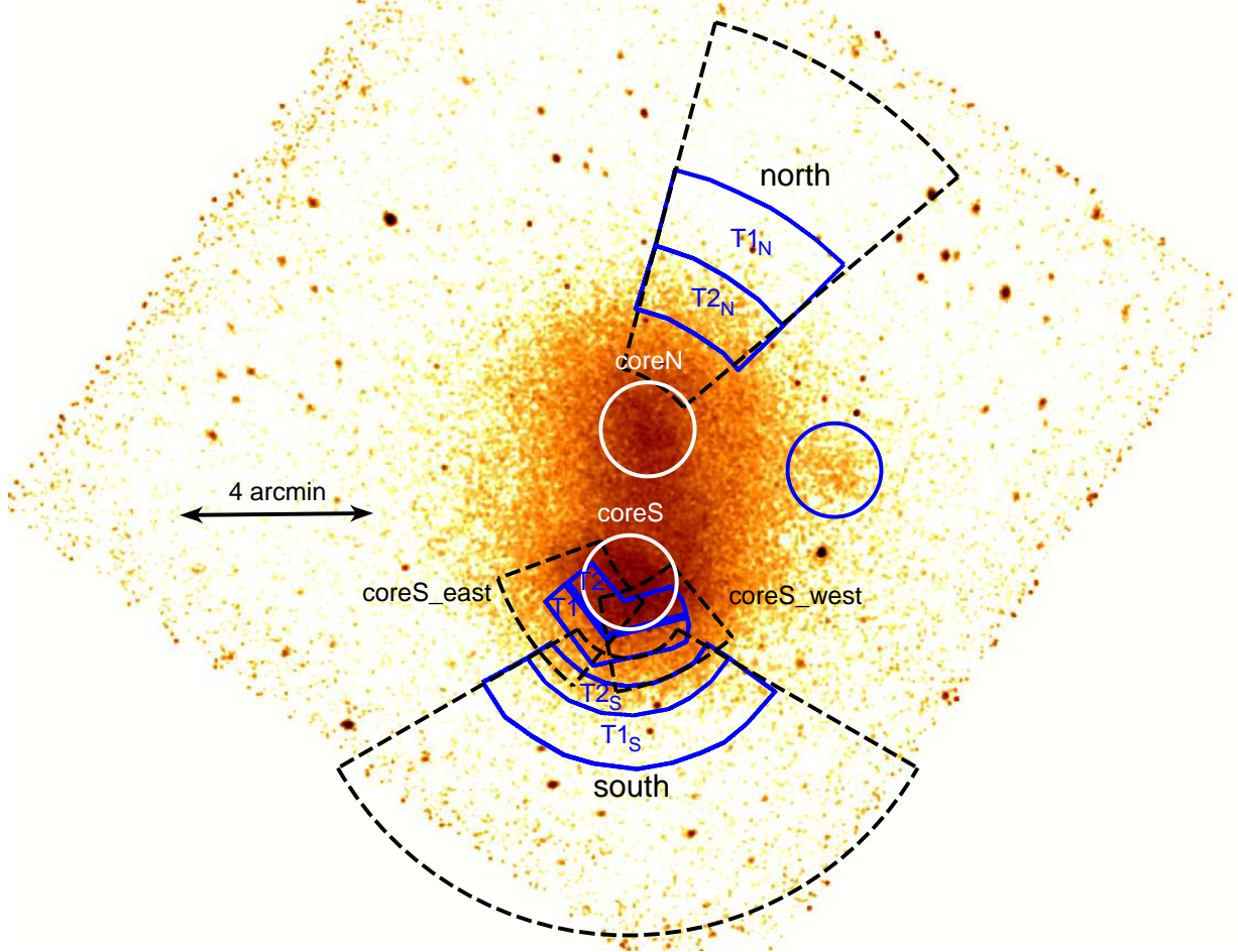
FIG. 12.— Smoothed (4 pixels) Chandra 0.5–2.0 keV image showing the sectors (dashed) in which we extracted and fitted the surface brightness profile, see Table 3. The regions where the temperatures ( T_1 and T_2 ) are extracted are shown in blue. The surface brightness edges are located at the boundary between the T_1 and T_2 regions. The blue circle represents the area where we extracted the X-ray luminosity of the western substructure. The white circles indicate the areas for which we extracted the temperatures for the cores of the northern ( coreN ) and southern ( coreS ) subclusters.
