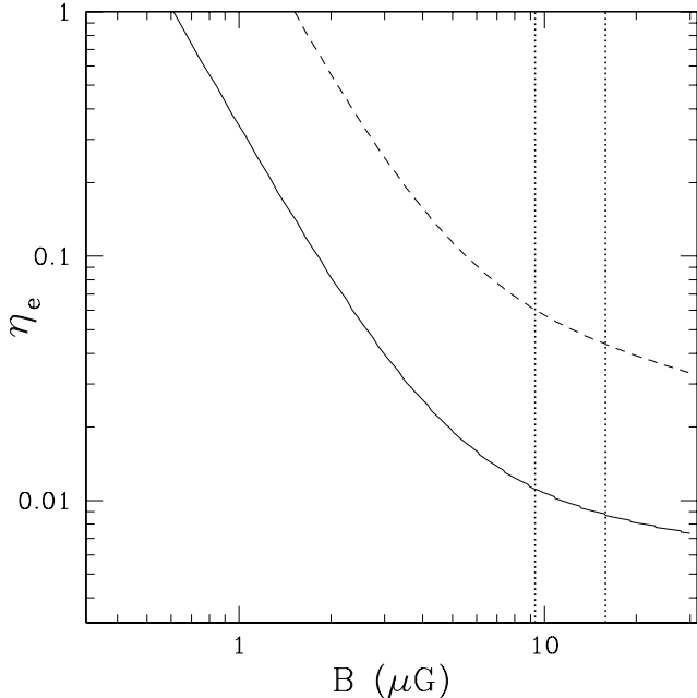
FIG. 15.— The fraction of the kinetic energy flux at the shock ( \eta_e ) that needs to be channelled into the supra-thermal and relativistic electron components that is required to explain the observed flux density of relic B1. The solid line is for \delta_{\text{inj}} = 2.2 and the dashed line for \delta_{\text{inj}} = 2.6 . For any reasonable value of the magnetic field strength ( B \lesssim 10 \mu\text{G} ) we find the extreme requirement that more than several percent of the kinetic energy flux crossing the shock should be converted into the acceleration of relativistic electrons. The two vertical dotted lines indicate the magnetic field value for plasma \beta values of 3 and 1.
