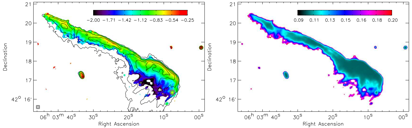
FIG. 5.— Left: Spectral index map between 151 and 610 MHz at 6.5'' resolution. Black contours are drawn at levels of [1, 2, 4, \dots] \times 1.25 \text{ mJy beam}^{-1} and are from the 151 MHz image. Pixels with values below 4.5\sigma_{\text{rms}} were blanked. The circled source at the western end of the relic is discussed in Sect. 5.3. Right: Corresponding spectral index error map. The errors are based on the individual r.m.s. noise levels in the two maps and using an absolute flux calibration uncertainty of 10% at 150 and 610 MHz.
