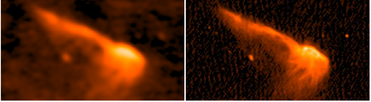
FIG. 4.— A comparison between the GMRT 150 MHz image (from van Weeren et al. 2012a), with a resolution of 26 \times 22'' , and the 120–181 MHz LOFAR image (from Figure 2), with a resolution of 4.8'' \times 3.9'' . The colors in both images were scaled manually to achieve similar image surface brightness levels. Except for the fine-scale structures, the images show very good agreement.
