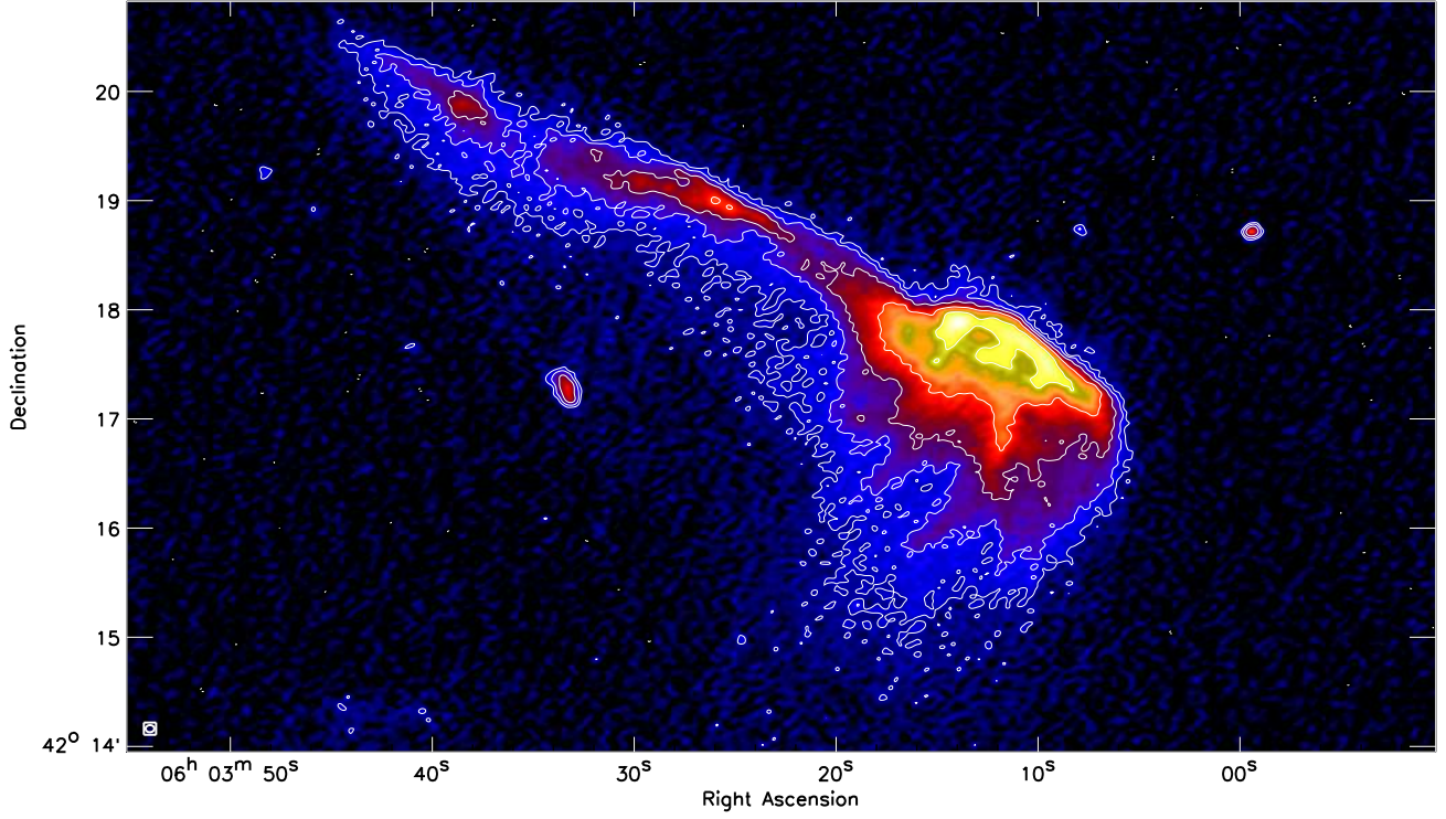
FIG. 2.— LOFAR HBA 120–181 MHz images made with robust=-1.5 (i.e., close to uniform) weighting of the visibilities. The beam size is 4.8'' \times 3.9'' and indicated in the bottom left corner. Contour levels are drawn at [1, 2, 4, 8, \dots] \times 4\sigma_{\text{rms}} , with \sigma_{\text{rms}} = 121 \mu\text{Jy beam}^{-1} .
