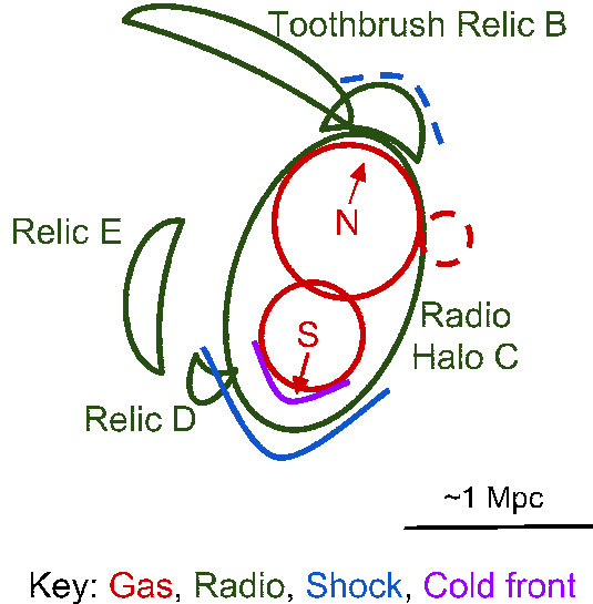
FIG. 10.— Schematic overview of the radio and X-ray components detected in the cluster. The dashed lines shows features whose identification is less certain.
