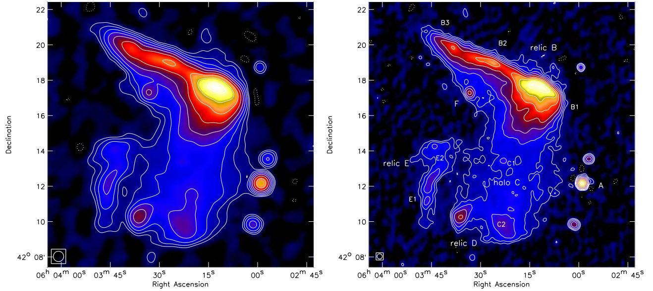
FIG. 3.— LOFAR HBA 120–181 MHz images with uniform weighting and uv-tapers of 40'' (left panel) and 20'' (right panel; sources are labelled as in Figure 1). The resulting beams are close to circular with sizes of 35.2'' and 17.7'' as indicated in the bottom left corner. Contour levels are drawn at [1, 2, 4, 8, \dots] \times 4\sigma_{\text{rms}} , with \sigma_{\text{rms}} = 358 and 212 \mu\text{Jy beam}^{-1} . Negative -3\sigma_{\text{rms}} contours are shown with dotted lines.
