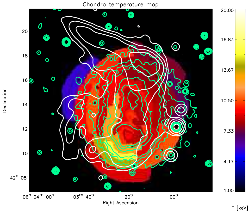
FIG. 11.— X-ray temperature map of the cluster. Each region was required to contain at least 5,000 net counts in the 0.5–7.0 keV band. X-ray contours (green) and radio contours (white, Figure 3 left panel) are overlaid. Black colored regions are blanked, either due to compact sources or because of an insufficient number of ICM counts.
