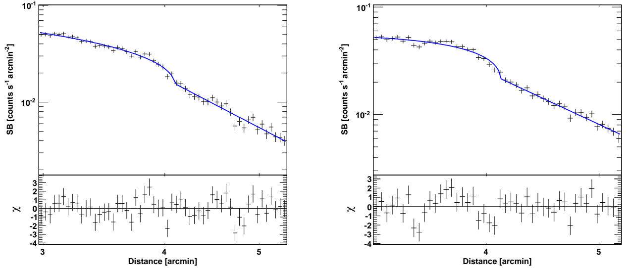
FIG. 14.— Left: X-ray surface brightness profiles for the right-angled edges around the southern cluster's core. The profile for the eastern sector is shown in the left panel and the western one in the right panel, see Figure 12. The blue lines show the best-fitting broken power-law density model (Eq. 1).
