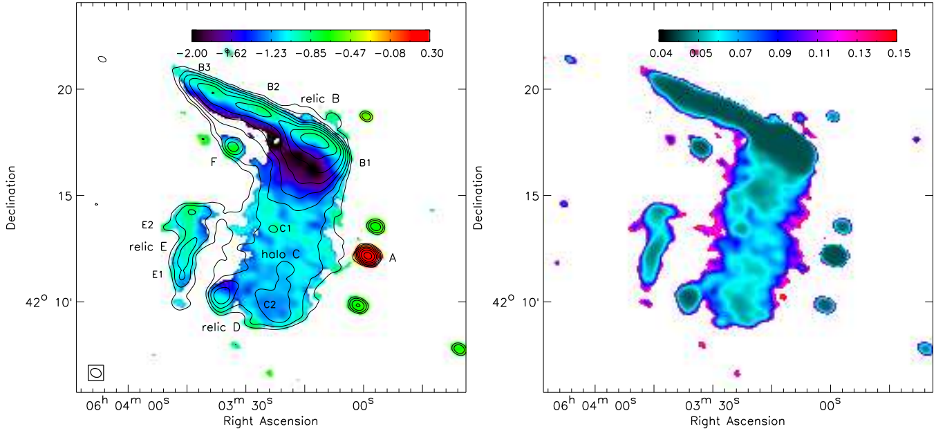
FIG. 7.— Left: Spectral index map between 0.151 and 1.5 GHz at 31'' \times 24'' resolution. Sources are labelled as in Figure 1). Black contours are drawn at levels of [1, 2, 4, \dots] \times 2 \text{ mJy beam}^{-1} and are from the 0.151 GHz image. Pixels with values below 3.5\sigma_{\text{rms}} were blanked. Right: Corresponding spectral index error map. The errors are based on the individual r.m.s. noise levels in the two maps and using an absolute flux calibration uncertainty of 10% at 150 MHz and 2.5% at 1.5 GHz.
