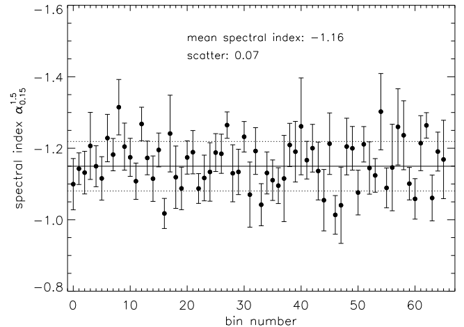
FIG. 16.— Spectral index distribution across the radio halo between 0.15 and 1.5 GHz in regions measuring 31 \text{ arcsec}^2 (see also Figure 7). The regions where the spectral indices are extracted, are indicated in the left panel of Figure 8 in blue. The solid horizontal line indicates the average spectral index. The dotted lines represent the measured scatter of the spectral indices. Systematic uncertainties in the flux-scale were not included in the error bars as they do not affect the measured scatter. The region (bin) numbering was randomized.
