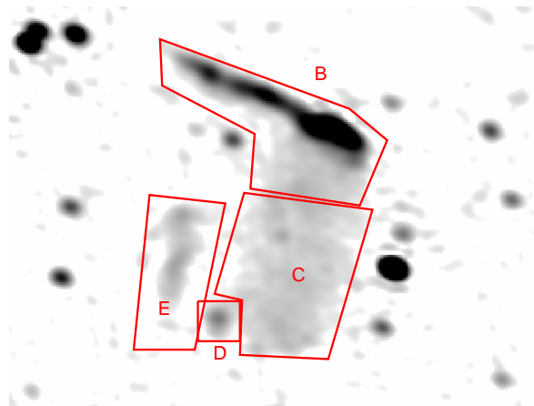
FIG. 18.— VLA 1–2 GHz images depicting the regions where the integrated flux densities were measured. The image has a resolution of 31'' \times 24'' .
