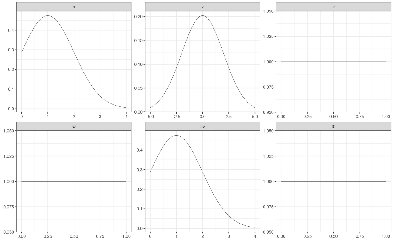
Figure 3 ■ An example of prior distributions.
