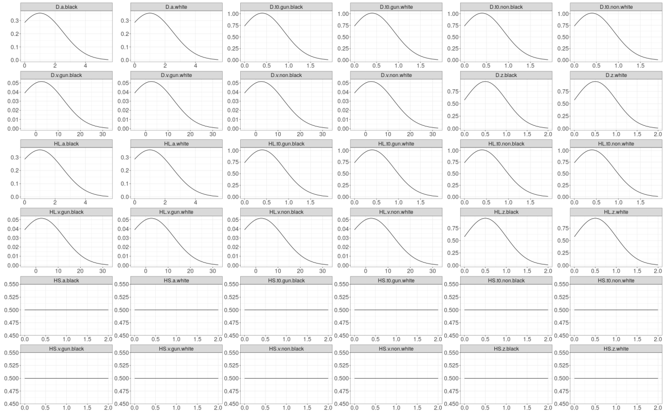
Figure 6 ■ Prior distributions. The base-level priors are shown under the strip titled, D.a.black, D.a.white, ..., D.z.white. D stands for the data-level priors. The location and the scale parameters of the hyper-level priors are represented by the HL and the HS, respectively. The x axis shows the value of the parameters and the y axis shows the probability densities.
