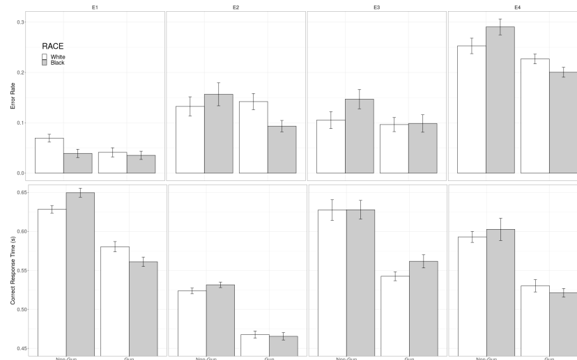
Figure 9 ■ Error rates and correct response times for the four studies reported in Pleskac, Cesario, and Johnson (2018). E1, E2, E3, and E4 represent experiment 1, 2, 3 and 4.
