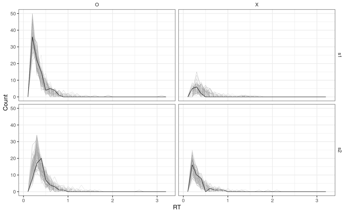
Figure 5 ■ The post-predictive probability density plots. O and X stand for the correct and incorrect responses. The two stimulus conditions are presented separately on the s1 and s2 rows (right y axis). Each grey line draws one posterior predictions based on the parameter estimates. The black line draws the data.
