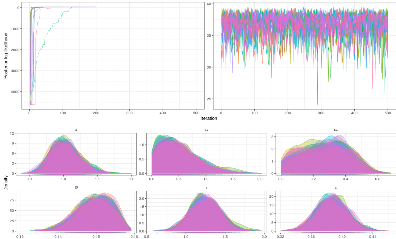
Figure 4 ■ Trace and probability density plots. Note the difference in the y axes. Different colors represent samples from different chains.
