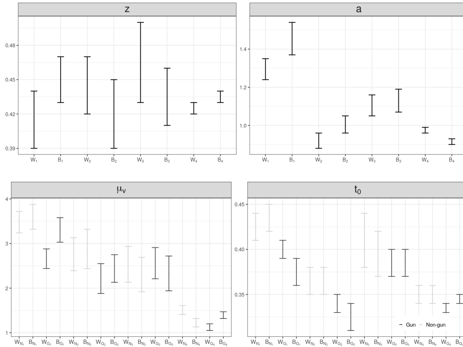
Figure 10 ■ The group-level parameter estimates of the Wiener diffusion model for each condition. The gray and dark lines are to highlight non-gun vs. gun objects (see the legend at the lower right corner). \mu_v and t_0 stands for drift rate and non-decision time. The error bars show 95% Bayesian credible intervals calculated from the posterior distributions.
