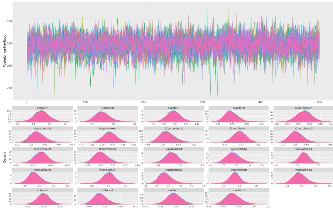
Figure 8 ■ Posterior trace and probability density plots.
