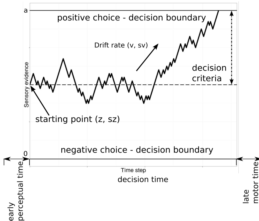
Figure 2 ■ An illustration of the diffusion decision model. The between-trial variabilities for the starting point, sz , and the drift rate, s_v , are grouped together with the main parameters, v and z . A positive choice ( a ) corresponds to, for instance a word stimulus with a word response. A negative choice ( 0 ) corresponds to a word stimulus with a non-word response. Non-decision time = early perceptual time + late motor time. RT = Non-decision time + decision time. The within-trial variability of the drift rate, the stochastic feature of the model, is illustrated by the wiggled line.
