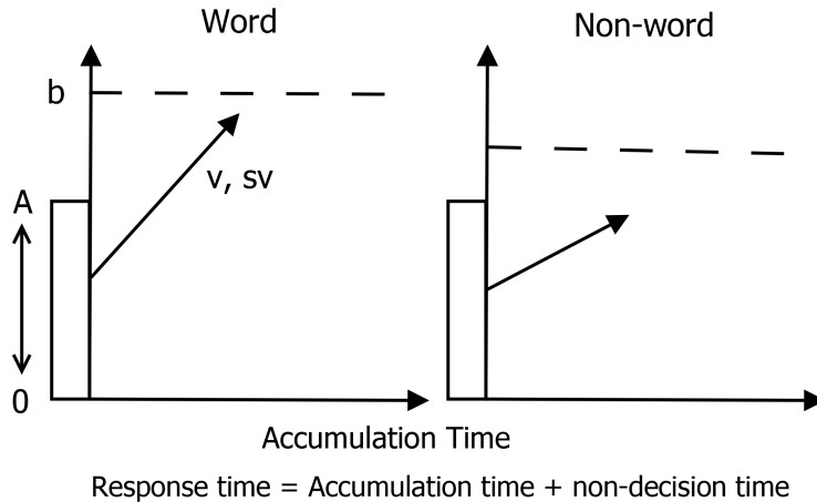
Figure 1 ■ An illustration of the linear ballistic accumulator model. Upon stimulus presentation, evidence accumulates towards each possible decision in parallel, and the first accumulator to reach threshold determines the observed response. Total RT is the time for the first accumulator to reach threshold plus non-decision time. A and b stand for the upper bound of the start-point noise and the response threshold. v and sv stand for the accumulation rate and its standard deviation. Figure adapted from Strickland, Loft, Remington, and Heathcote (2018).
