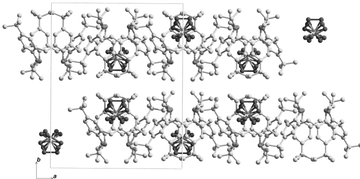
FIGURE 4. The crystal packing of 2 \cdot \text{CHCl}_3 projected down c .
