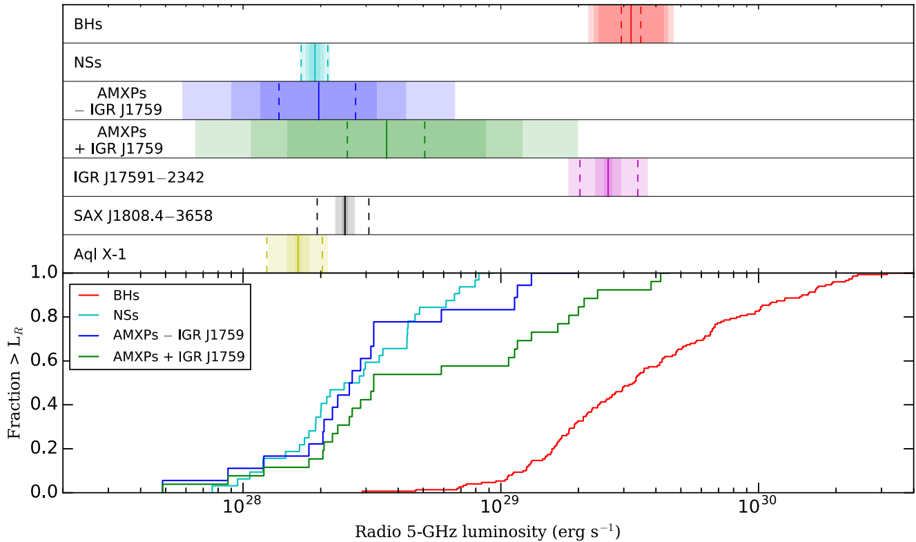
Figure 3. Top: Inferred parameters of the LINMIX_ERR fit (equation 1) to X-ray and radio luminosities of different classes of NS-LMXB and BH-LMXB, as well as individual sources (using an X-ray luminosity range 4 \times 10^{35} \text{ erg s}^{-1} < L_X < 10^{37} \text{ erg s}^{-1} ). The solid and dashed lines represent values of the radio luminosity intercept \xi + L_{R,c} and its uncertainties, respectively. The shaded areas represent the intrinsic scatter \sigma_0 of radio luminosities around the best-fitting function of the slope, along with its uncertainties. Bottom: Cumulative distribution function for 5-GHz radio luminosities of different classes of NS-LMXB and BH-LMXB.
