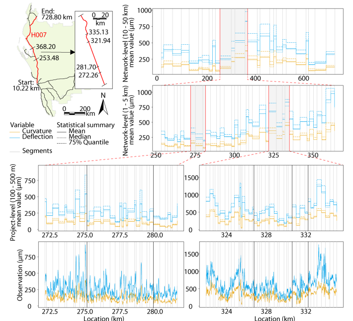
Fig. 5. Statistical comparison of project- and network-level segments derived by the SHS method
