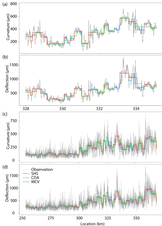
Fig. 7. Visualization comparison of three homogeneous segmentation methods: SHS, CDA, and MCV, for project-level (100–500 m) segments ((a) curvature segments, and (b) deflection) and network-level (1–5 km) segments ((c) curvature and (d) deflection) in parts of the road network
