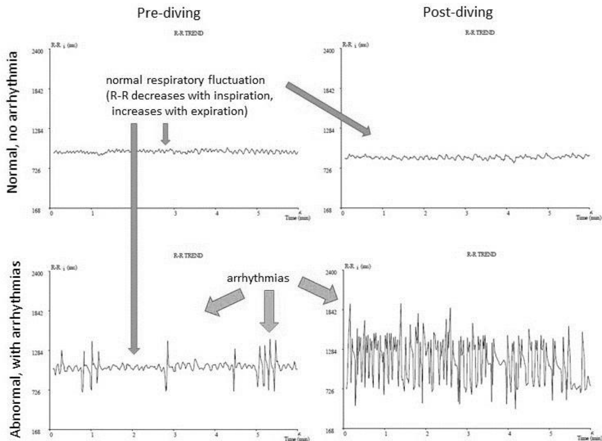
Figure 3: Examples of beat-to-beat (R-R) interval (ms) trends of divers before vs after dive trips, 360 sec (6 min) recordings
