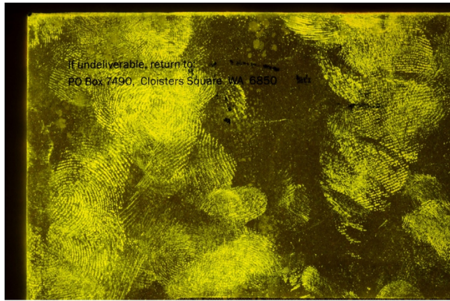
Fig. 7. Example of latent fingerprints developed with IND/Zn on a contemporaneous envelope.
