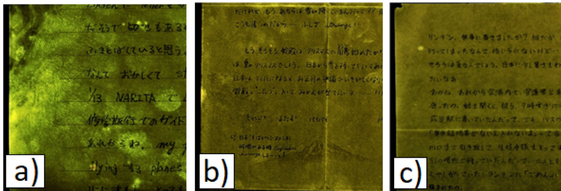
Fig. 1. Example of developed fingermarks on documents dating back to 1980, showing potentially identifiable fingermarks (a), evidence of handling (b) and no fingermarks (c).
