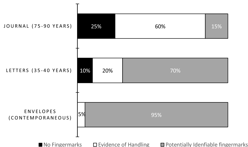
Fig. 8. Percentage results of the characterisation of documents of different ageing periods based on the quality of fingerprints developed after treatment with IND/Zn under Australian climatic conditions.
