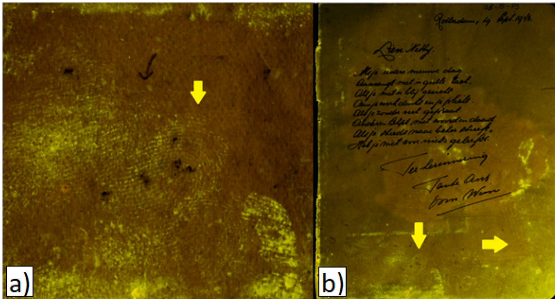
Fig. 3. Potentially identifiable fingermark (a), and diffuse features possibly associated with original areas of contact (b), developed with IND/Zn on a journal dating back to 1940s.
