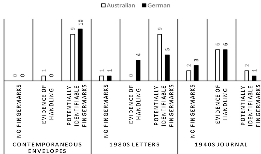
Fig. 9. Comparison between Australian and German IND/Zn formulations based on the best quality fingermarks developed on three sets of documents of different ageing periods.
