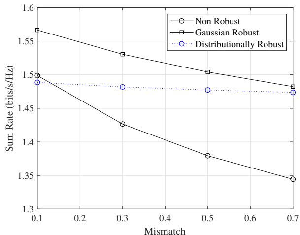
Fig. 10: Example 2: Sum rate versus the CSI mismatch level \nu .
