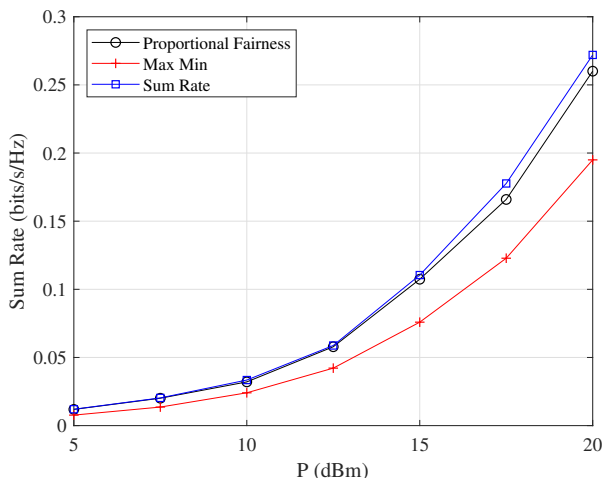
Fig. 6: Example 1: Sum rate versus P , \sigma^2 = -90 dBm and \varpi_0 = -30 dB.
