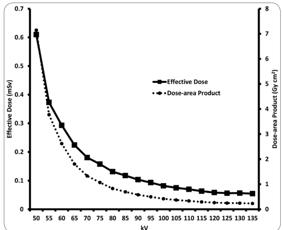
Figure 3. Effect of tube voltage on radiation doses.
