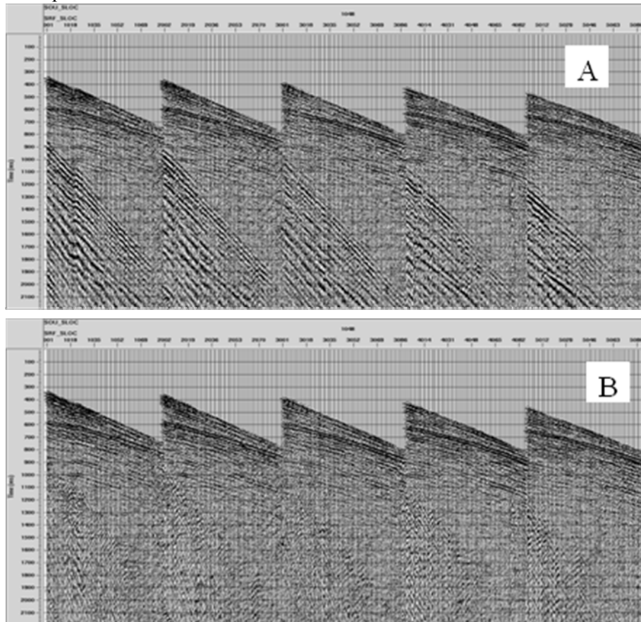
Figure 2 Before (A) and after (B) removal of source generated filter by Radon filter. Top display is weight drop data, bottom vibroseis data.
