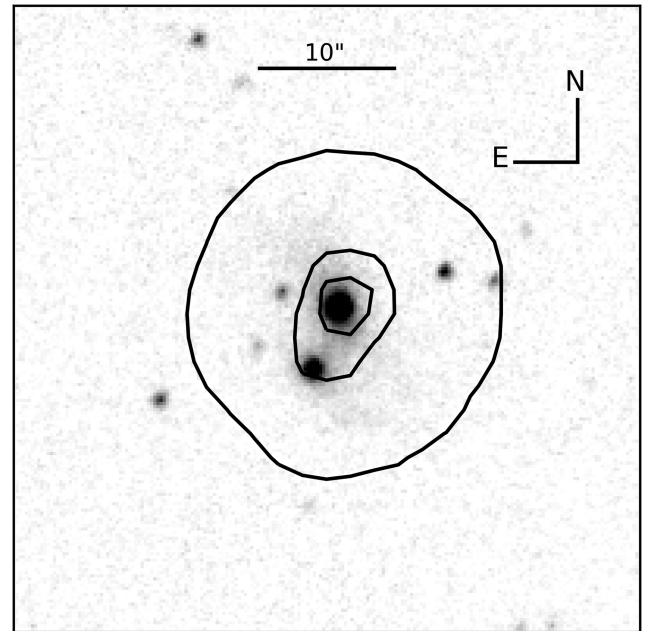
Figure 11. NOT K_s -band image of IRAS 23436+5257 from 2017 July 27 with 24 \mu\text{m} MIPS contours overplotted. The 24 \mu\text{m} emission is concentrated on the Northern nucleus, supporting it as a potential AGN host.
