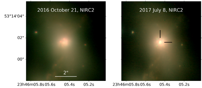
Figure 1. AT 2017gbl coincident with the Northern nucleus of IRAS 23436+5257, discovered with NIRC2. Left-hand panel shows a JHK_s colour composite from the NIRC2 template epoch in 2016 October. Right-hand panel shows a JHK_s colour-composite of the discovery epoch of AT 2017gbl in 2017 July. Image cutouts are \sim 7.5 arcsec across.
