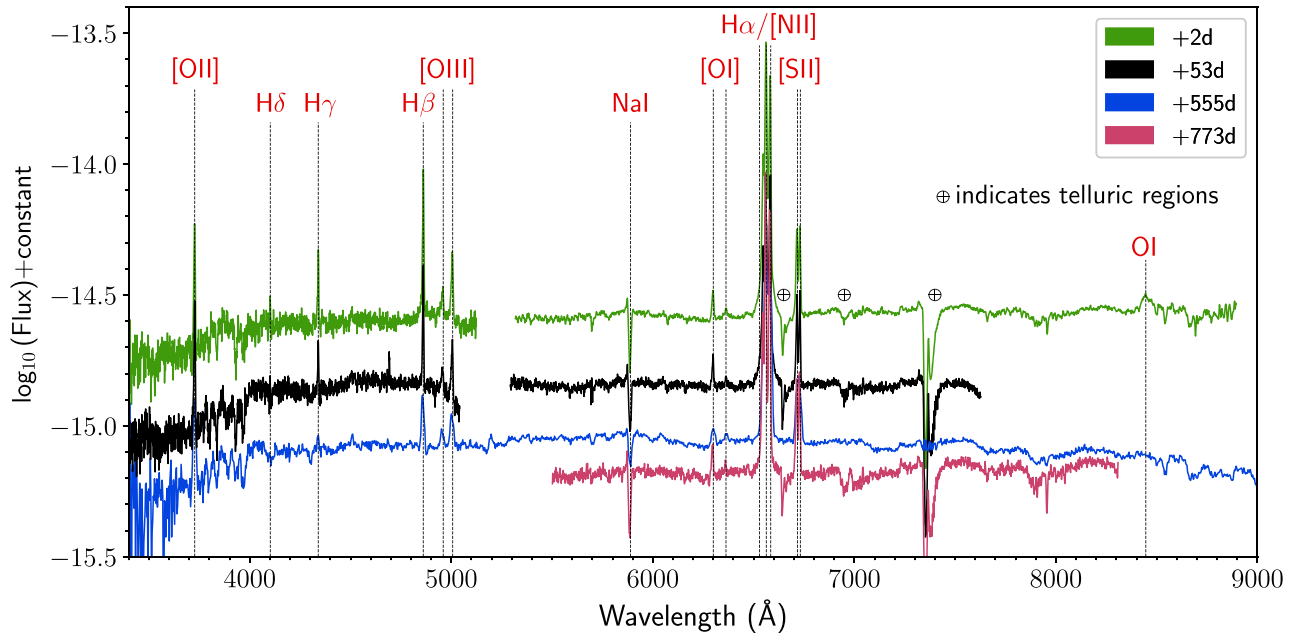
Figure 6. Optical follow-up spectra of AT 2017gbl. Spectra are corrected for Milky Way reddening. Some emission and absorption features are indicated. Note the broad OI feature at 8446 Å that is present initially but not in late observations. Note that the broadening of the narrow lines in the spectrum taken at +555 d is because the data are from a lower resolution instrument.
