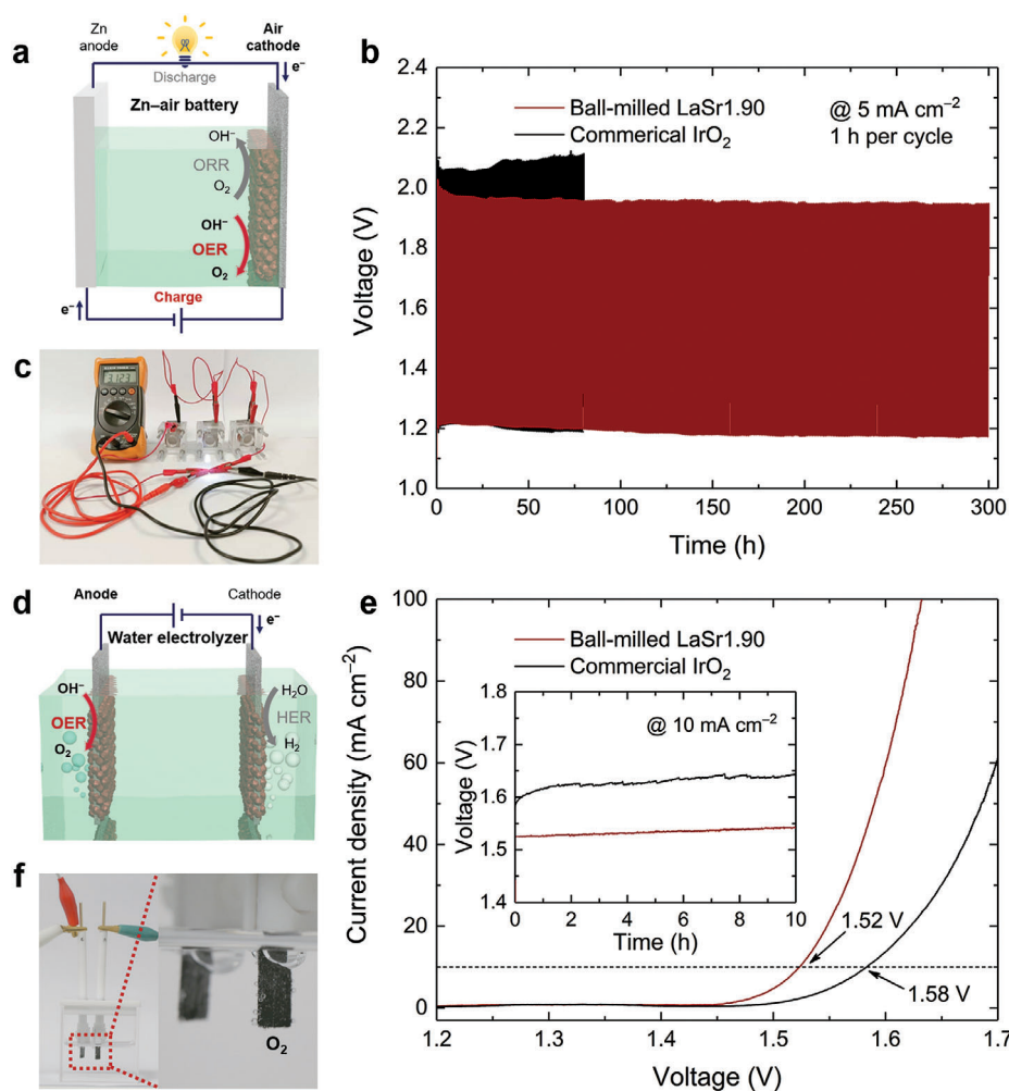
Figure 5. Evaluation of the electrochemical performance of the ball-milled LaSr 1.90 sample in a rechargeable Zn–air battery and a water electrolyzer. a) Schematic illustration of a rechargeable Zn–air battery. ORR: oxygen reduction reaction. b) Galvanostatic charge/discharge profiles of Zn–air batteries using the ball-milled LaSr 1.90 and the commercial IrO 2 catalysts at 5 mA cm -2 (electrolyte: 6 M KOH + 0.2 M zinc acetate). c) Photograph showing how three Zn–air batteries assembled in series could power a light-emitting diode. d) Schematic illustration of a water electrolyzer. HER: hydrogen evolution reaction. e) Polarization curves of water electrolyzers using the ball-milled LaSr 1.90 and the commercial IrO 2 , respectively, as anode catalyst and commercial 20 wt% Pt/C as cathode catalyst (electrolyte: 1 M KOH). Inset shows the chronopotentiometry curves at 10 mA cm -2 . f) Photograph showing how the water electrolyzer could continuously generate gas bubbles during the stability test.
