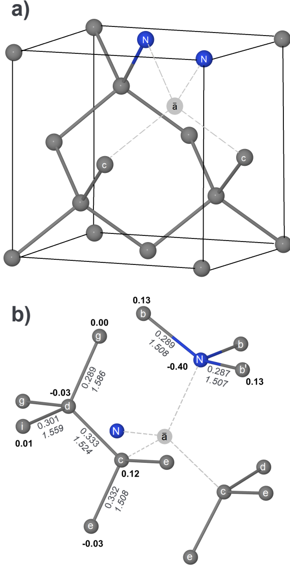
FIG. 11. The VN 2 0 defect. In panel a) the pristine diamond conventional cell is shown, whereas in panel b) a local cluster of C and N atoms adjacent to the vacancy and including 12 next-nearest neighbors is represented. Mulliken net charges (in |e| units; boldface) are shown near the atoms, for each symmetry irreducible atom. Bond distances (in Å, italics) and Mulliken bond populations (in |e|) are also shown in between the two involved atoms. Data refer to the doublet ground spin state.
