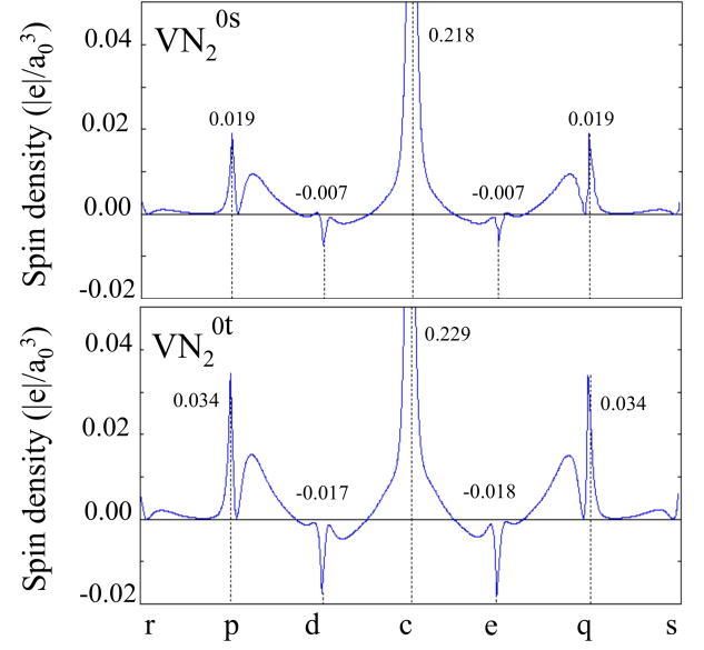
FIG. 12. Spin density profiles of the VN 2 0 defect in its singlet (top) and triplet (bottom) spin states along a path connecting the atoms with relatively high spin density. Some of the atomic labels appear in panel b) of figure 11, others refer to atoms connected to atoms at the border of the reported cluster. All calculations were done with the S 216 supercell, B3LYP functional and the 6-31G-J* basis set. 175
