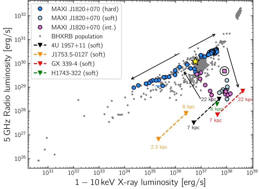
Figure 1 | The radio–X-ray correlation for the BHXRb population and J1820. Radio luminosity as a function of X-ray luminosity for J1820, based on our monitoring at 15.5 GHz with the AMI-LA radio Telescope (scaled to 5 GHz assuming a flat spectrum) and X-ray observations from the Swift X-ray telescope. The data for J1820 in the hard state, soft state and intermediate state are shown by dark blue circles, light blue diamonds and purple squares, respectively. For the majority of data points the error bars are too small to be seen. The yellow star marks our first simultaneous radio/X-ray observation of J1820 (3.2 d after our first radio observation) and the black arrows show schematically the time evolution of the outburst. We only use X-ray observations within 8 h of our radio observations, with the exception of the purple square circumscribed with a circle. In this case the observations were taken \sim 14 h apart. Error bars on data points indicate one sigma uncertainties. Data from the literature on other black hole systems are indicated by grey dots 44 . We mark upper limits for core soft state emission from the XRB systems 4U 1957+11, J1753.5–0127, GX 339–4 and H1743–322 8–10,45 for a range of possible distances. We do not include radio observations taken during the state transition flare. We use a distance of 3.1 kpc when calculating the luminosities 31 .
