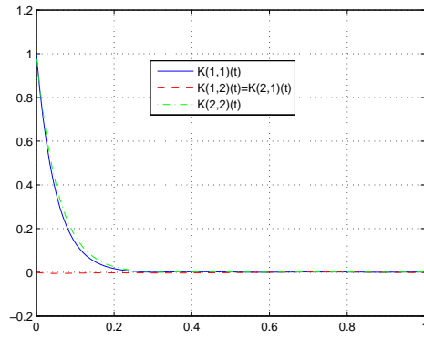
FIGURE 2. The state K^*(t) with N = 5 .
