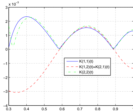
FIGURE 2. The state K^*(t) with N = 5 .
