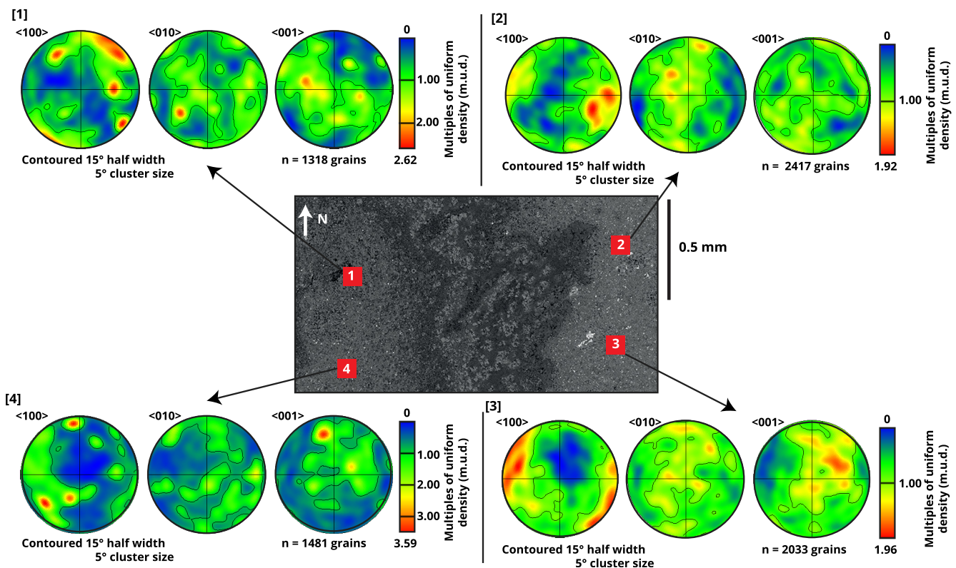
FIGURE 5. Contoured lower hemisphere, equal area plots from high-resolution maps surrounding the calcium-aluminum inclusions [1–4]. All data were contoured with a half width of 15^\circ and a cluster size of 5^\circ . Center reference image is backscatter electron map, adapted from Forman et al. (2019). (Color figure can be viewed at wileyonlinelibrary.com .)
