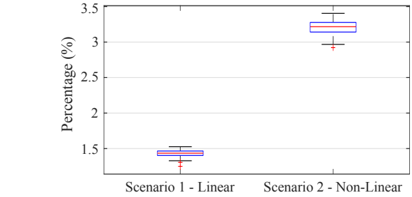
Fig. 5. Percentage of the smooth trajectory estimator's computational time in relation to the total filtering time averaged over 100 Monte Carlo trials.
