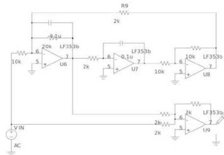
Figure 1 - Circuit for Construction and Test
